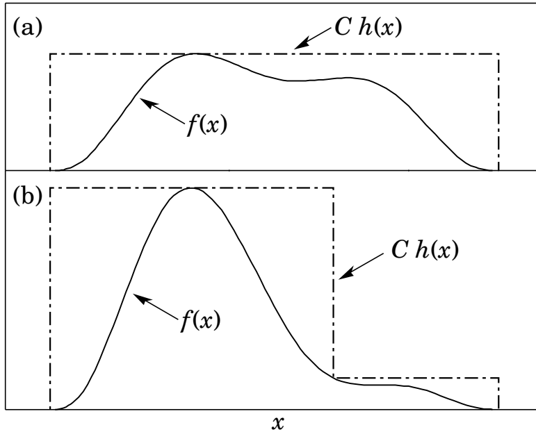
Figure 39.2: Illustration of the acceptance-rejection method. Random points are chosen inside the upper bounding figure, and rejected if the ordinate exceeds f(x) . The lower figure illustrates a method to increase the efficiency (see text).
