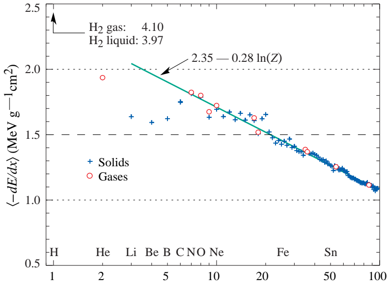
Figure 32.3: Stopping power at minimum ionization for the chemical elements. The straight line is fitted for Z > 6 . A simple functional dependence on Z is not to be expected, since \langle -dE/dx \rangle also depends on other variables.
