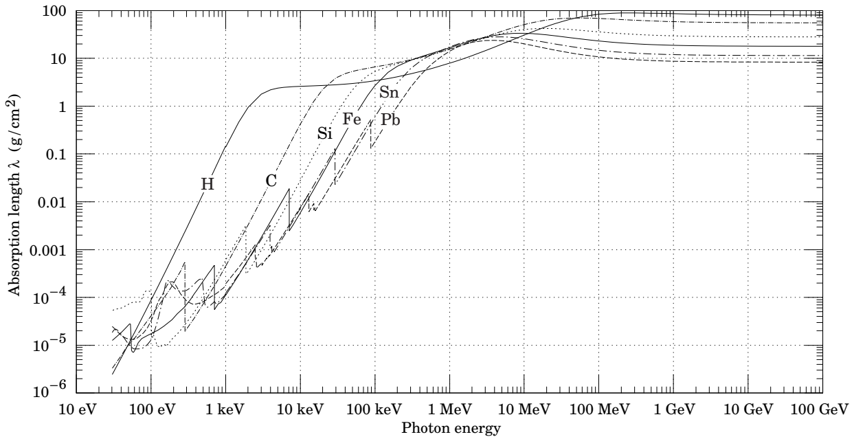
Figure 32.16: The photon mass attenuation length (or mean free path) \lambda = 1/(\mu/\rho) for various elemental absorbers as a function of photon energy. The mass attenuation coefficient is \mu/\rho , where \rho is the density. The intensity I remaining after traversal of thickness t (in mass/unit area) is given by I = I_0 \exp(-t/\lambda) . The accuracy is a few percent. For a chemical compound or mixture, 1/\lambda_{\text{eff}} \approx \sum_{\text{elements}} w_Z/\lambda_Z , where w_Z is the proportion by weight of the element with atomic number Z . The processes responsible for attenuation are given in Fig. 32.11. Since coherent processes are included, not all these processes result in energy deposition. The data for 30 \text{ eV} < E < 1 \text{ keV} are obtained from http://www-cxro.lbl.gov/optical_constants (courtesy of Eric M. Gullikson, LBNL). The data for 1 \text{ keV} < E < 100 \text{ GeV} are from http://physics.nist.gov/PhysRefData , through the courtesy of John H. Hubbell (NIST).
