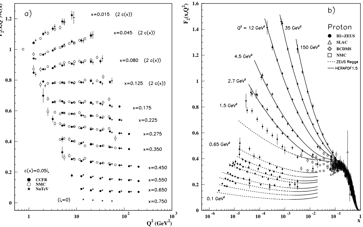
Figure 19.10: a) The deuteron structure function F_2 measured in deep inelastic scattering of muons on a fixed target (NMC) is compared to the structure function F_2 from neutrino-iron scattering (CCFR and NuTeV) using F_2^{\mu} = (5/18)F_2^{\nu} - x(s + \bar{s})/6 , where heavy-target effects have been taken into account. The data are shown versus Q^2 , for bins of fixed x . The NMC data have been rebinned to CCFR and NuTeV x values. For the purpose of plotting, a constant c(x) = 0.05i_x is added to F_2 , where i_x is the number of the x bin, ranging from 0 ( x = 0.75 ) to 7 ( x = 0.175 ). For i_x = 8 ( x = 0.125 ) to 11 ( x = 0.015 ), 2c(x) has been added. References: NMC —M. Arneodo et al. , Nucl. Phys. B483 , 3 (1997); CCFR/NuTeV —U.K. Yang et al. , Phys. Rev. Lett. 86 , 2741 (2001); NuTeV —M. Tzanov et al. , Phys. Rev. D74 , 012008 (2006).
