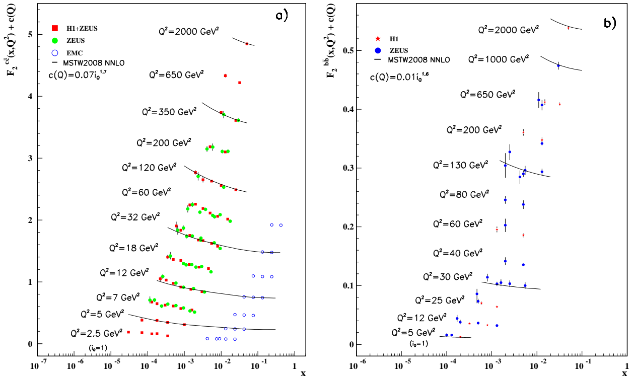
Figure 19.11: a) The charm-quark structure function F_2^{c\bar{c}}(x) , i.e. that part of the inclusive structure function F_2^D arising from the production of charm quarks, measured in electromagnetic scattering of positrons on protons (H1, ZEUS) and muons on iron (EMC). For the purpose of plotting, a constant c(Q) = 0.07i_Q^{1.7} is added to F_2^{c\bar{c}} where i_Q is the number of the Q^2 bin, ranging from 1 ( Q^2 = 2.5 \text{ GeV}^2 ) to 12 ( Q^2 = 2000 \text{ GeV}^2 ). References: H1 and ZEUS run I combination —H. Abramowicz et al. , Eur. Phys. J. C73 , 2311 (2013); ZEUS run II —H. Abramowicz et al. , JHEP 05 , 023 (2013); H. Abramowicz et al. , JHEP 05 , 097 (2013); EMC —J.J. Aubert et al. , Nucl. Phys. B213 , 31 (1983).
