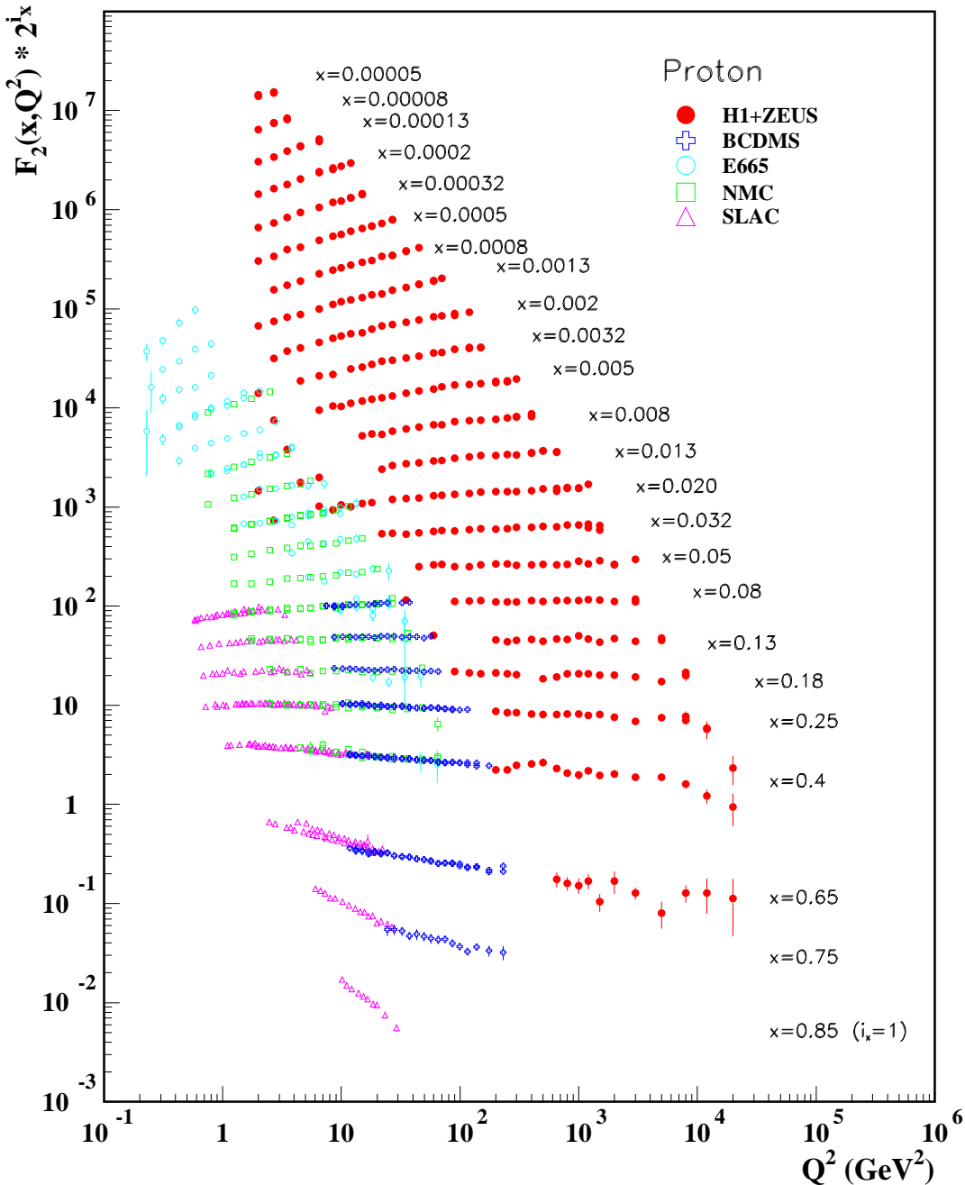
Figure 19.8: The proton structure function F_2^p measured in electromagnetic scattering of electrons and positrons on protons (collider experiments H1 and ZEUS for Q^2 \geq 2 GeV ^2 ), in the kinematic domain of the HERA data (see Fig. 19.10 for data at smaller x and Q^2 ), and for electrons (SLAC) and muons (BCDMS, E665, NMC) on a fixed target. Statistical and systematic errors added in quadrature are shown. The data are plotted as a function of Q^2 in bins of fixed x . Some points have been slightly offset in Q^2 for clarity. The H1+ZEUS combined binning in x is used in this plot; all other data are rebinned to the x values of these data. For the purpose of plotting, F_2^p has been multiplied by 2^{i_x} , where i_x is the number of the x bin, ranging from i_x = 1 ( x = 0.85 ) to i_x = 24 ( x = 0.00005 ). References: H1 and ZEUS —F.D. Aaron et al. , JHEP 1001 , 109 (2010); BCDMS —A.C. Benvenuti et al. , Phys. Lett. B223 , 485 (1989) (as given in [78]) ; E665 —M.R. Adams et al. , Phys. Rev. D54 , 3006 (1996); NMC —M. Arneodo et al. , Nucl. Phys. B483 , 3 (1997); SLAC —L.W. Whitlow et al. , Phys. Lett. B282 , 475 (1992).
