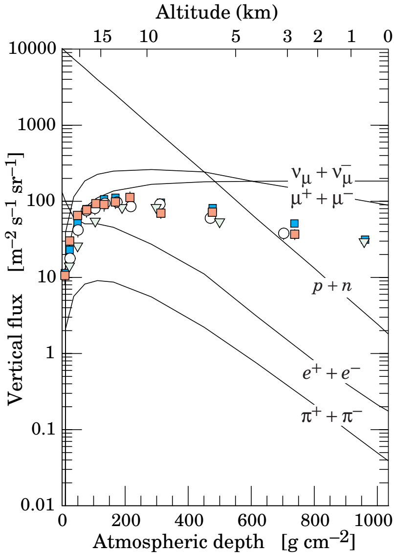
Figure 28.4: Vertical fluxes of cosmic rays in the atmosphere with E > 1 GeV estimated from the nucleon flux of Eq. (28.2). The points show measurements of negative muons with E_\mu > 1 GeV [41–45].
