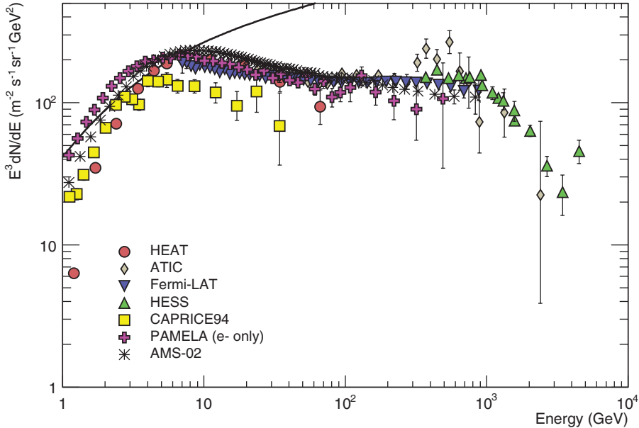
Figure 28.2: Differential spectrum of electrons plus positrons (except PAMELA data, which are electrons only) multiplied by E^3 [19–23,33,34]. The line shows the proton spectrum [25] multiplied by 0.01.
