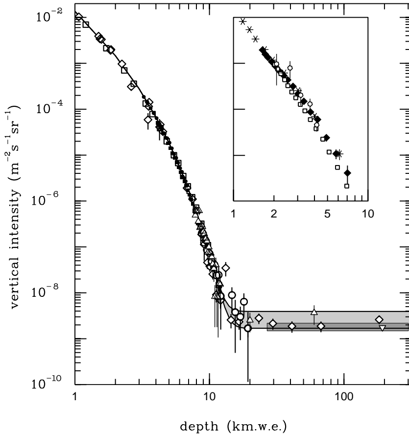
Figure 28.7: Vertical muon intensity vs depth (1 km.w.e. = 10^5 g cm ^{-2} of standard rock). The experimental data are from: \diamond : the compilations of Crouch [69], \square : Baksan [74], \circ : LVD [75], \bullet : MACRO [76], \blacksquare : Frejus [77], and \triangle : SNO [78]. The shaded area at large depths represents neutrino-induced muons of energy above 2 GeV. The upper line is for horizontal neutrino-induced muons, the lower one for vertically upward muons. Darker shading shows the muon flux measured by the SuperKamiokande experiment. The inset shows the vertical intensity curve for water and ice published in Refs. [70–73].
