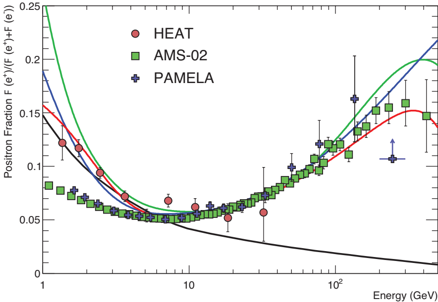
Figure 28.3: The positron fraction (ratio of the flux of e^+ to the total flux of e^+ and e^- ) [26,24,30]. The heavy black line is a model of pure secondary production [28] and the three thin lines show three representative attempts to model the positron excess with different phenomena: green: dark matter decay [29]; blue: propagation physics [32]; red: production in pulsars [40]. The ratio below 10 GeV is dependent on the polarity of the solar magnetic field.
