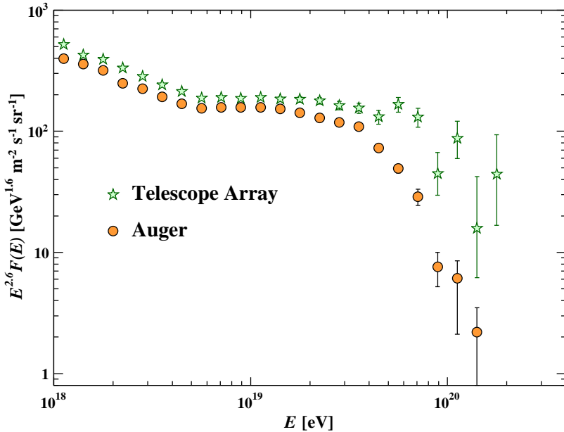
Figure 28.9: Expanded view of the highest energy portion of the cosmic-ray spectrum from data of the Telescope Array [104], and the Auger Observatory [105].
