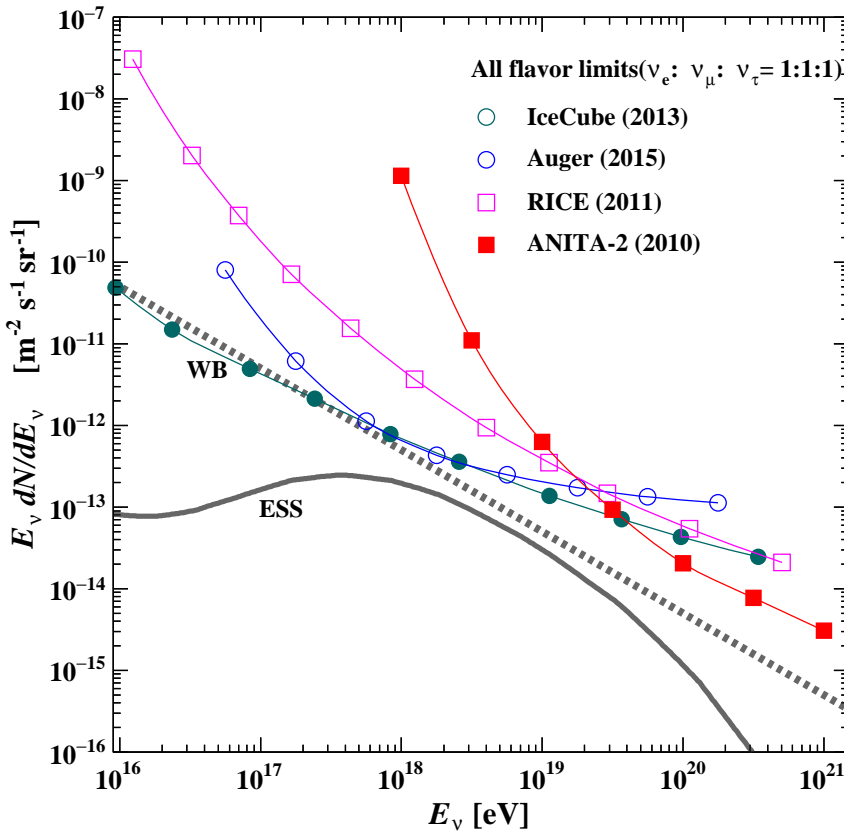
Figure 28.10: Differential limits on the flux of cosmogenic neutrinos set by four neutrino experiments. The curves show the Waxman-Bahcall benchmark flux (WB, [124]) and a representative midrange model for the expected flux of cosmogenic neutrinos (ESS, [123]). The expected flux is uncertain by over an order of magnitude in either direction.
