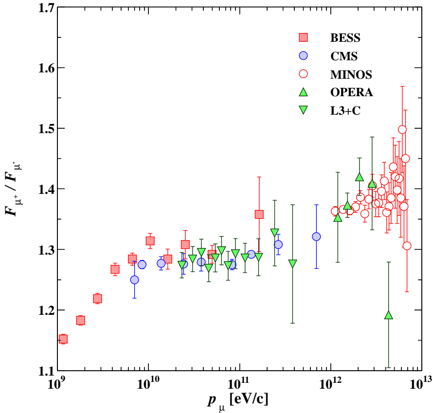
Figure 28.6: Muon charge ratio as a function of the muon momentum from Refs. [53,54,60,65,66].
