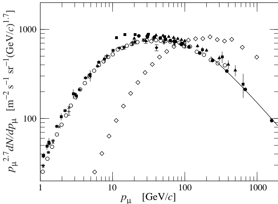
Figure 28.5: Spectrum of muons at \theta = 0^\circ ( \diamond [50], \blacksquare [56], \blacktriangledown [57], \blacktriangle [58], \times , + [52], \circ [53], and \bullet [54] and \theta = 75^\circ \diamond [59]). The line plots the result from Eq. (28.4) for vertical showers.
