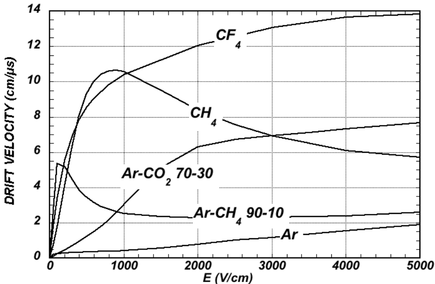
Figure 33.4: Computed electron drift velocity as a function of electric field in several gases at NTP and B = 0 [71].
