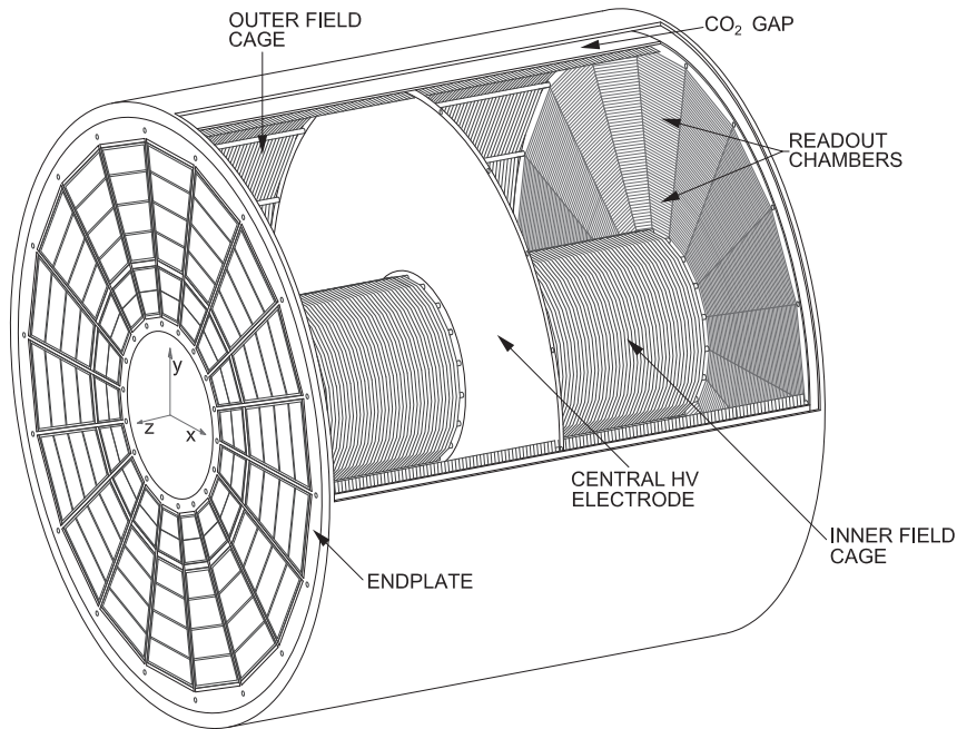
Figure 33.13: Schematic view of the ALICE TPC [106]. The drift volume with 5 m diameter is divided into two halves, each providing 2.5 m drift length.
