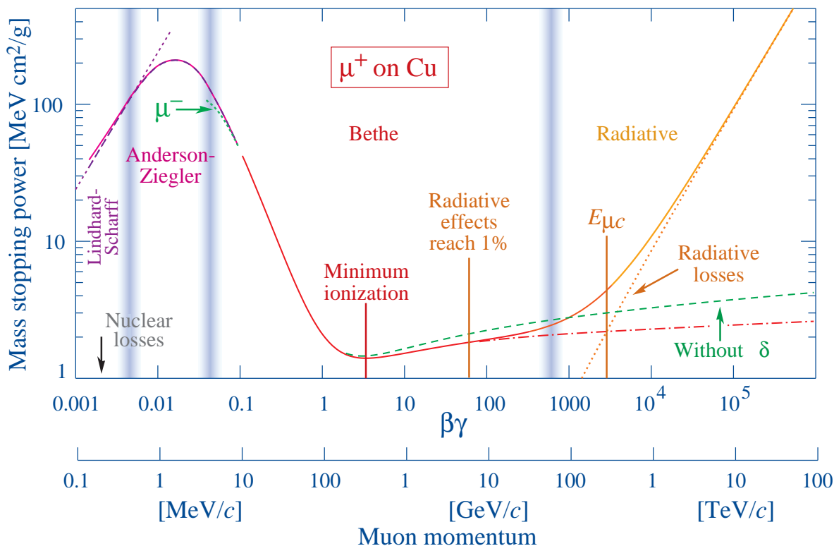
Fig. 32.1: Mass stopping power ( = \langle -dE/dx \rangle ) for positive muons in copper as a function of \beta\gamma = p/Mc over nine orders of magnitude in momentum (12 orders of magnitude in kinetic energy). Solid curves indicate the total stopping power. Data below the break at \beta\gamma \approx 0.1 are taken from ICRU 49 [4], and data at higher energies are from Ref. 5. Vertical bands indicate boundaries between different approximations discussed in the text. The short dotted lines labeled “ \mu^- ” illustrate the “Barkas effect,” the dependence of stopping power on projectile charge at very low energies [6]. dE/dx in the radiative region is not simply a function of \beta .
