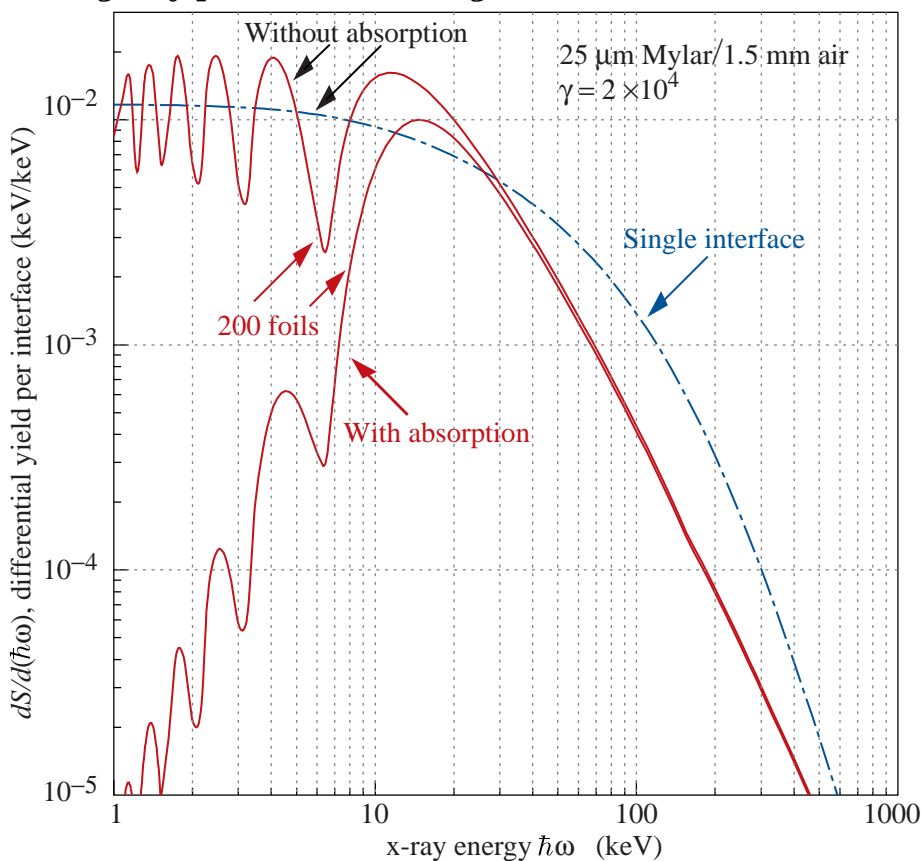
Figure 32.27: X-ray photon energy spectra for a radiator consisting of 200 25\ \mu\text{m} thick foils of Mylar with 1.5 mm spacing in air (solid lines) and for a single surface (dashed line). Curves are shown with and without absorption. Adapted from Ref. 88.
