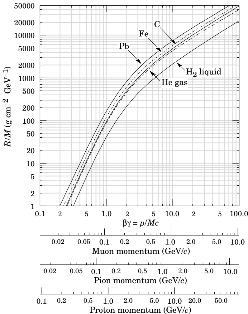
Figure 32.4: Range of heavy charged particles in liquid (bubble chamber) hydrogen, helium gas, carbon, iron, and lead. For example: For a K^+ whose momentum is 700 \text{ MeV}/c , \beta\gamma = 1.42 . For lead we read R/M \approx 396 , and so the range is 195 \text{ g cm}^{-2} (17 cm).
