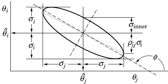
Figure 38.5: Standard error ellipse for the estimators \hat{\theta}_i and \hat{\theta}_j . In the case shown the correlation is negative.
