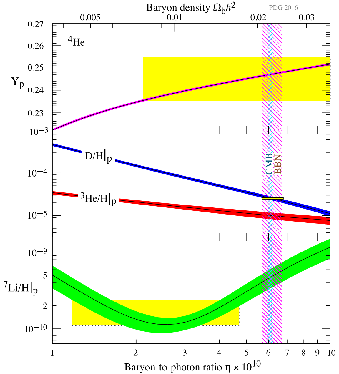
Figure 23.1: The primordial abundances of {}^4\text{He} , \text{D} , {}^3\text{He} , and {}^7\text{Li} as predicted by the standard model of Big-Bang nucleosynthesis—the bands show the 95% CL range [5]. Boxes indicate the observed light element abundances. The narrow vertical band indicates the CMB measure of the cosmic baryon density, while the wider band indicates the BBN concordance range (both at 95% CL).
