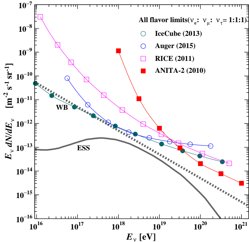
Figure 28.10: Differential limits on the flux of cosmogenic neutrinos set by four neutrino experiments. The curves show the Waxman-Bahcall benchmark flux (WB, [124]) and a representative midrange model for the expected flux of cosmogenic neutrinos (ESS, [123]). The expected flux is uncertain by over an order of magnitude in either direction.
