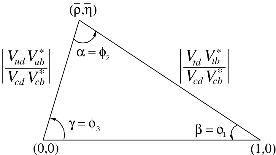
Figure 12.1: Sketch of the unitarity triangle.
