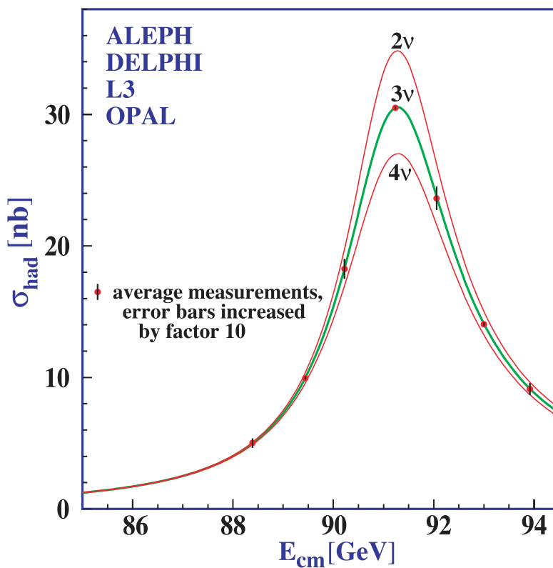
Figure 51.7: Combined data from the ALEPH, DELPHI, L3, and OPAL Collaborations for the cross section in e^+e^- annihilation into hadronic final states as a function of the center-of-mass energy near the Z pole. The curves show the predictions of the Standard Model with two, three, and four species of light neutrinos. The asymmetry of the curve is produced by initial-state radiation. Note that the error bars have been increased by a factor ten for display purposes. References:
