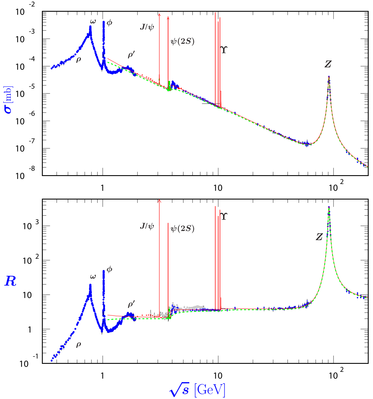
Figure 51.5: World data on the total cross section of e^+e^- \rightarrow \text{hadrons} and the ratio R(s) = \sigma(e^+e^- \rightarrow \text{hadrons}, s) / \sigma(e^+e^- \rightarrow \mu^+\mu^-, s) . \sigma(e^+e^- \rightarrow \text{hadrons}, s) is the experimental cross section corrected for initial state radiation and electron-positron vertex loops, \sigma(e^+e^- \rightarrow \mu^+\mu^-, s) = 4\pi\alpha^2(s)/3s . Data errors are total below 2 GeV and statistical above 2 GeV. The curves are an educative guide: the broken one (green) is a naive quark-parton model prediction, and the solid one (red) is 3-loop pQCD prediction (see “Quantum Chromodynamics” section of this Review, Eq. (9.7) or, for more details, K. G. Chetyrkin et al. , Nucl. Phys. B586 , 56 (2000) (Erratum ibid. B634 , 413 (2002))). Breit-Wigner parameterizations of J/\psi , \psi(2S) , and \Upsilon(nS) , n = 1, 2, 3, 4 are also shown. The full list of references to the original data and the details of the R ratio extraction from them can be found in [arXiv:hep-ph/0312114]. Corresponding computer-readable data files are available at http://pdg.lbl.gov/current/xsect/ . (Courtesy of the COMPAS (Protvino) and HEPDATA (Durham) Groups, August 2015. Corrections by P. Janot (CERN) and M. Schmitt (Northwestern U.))
