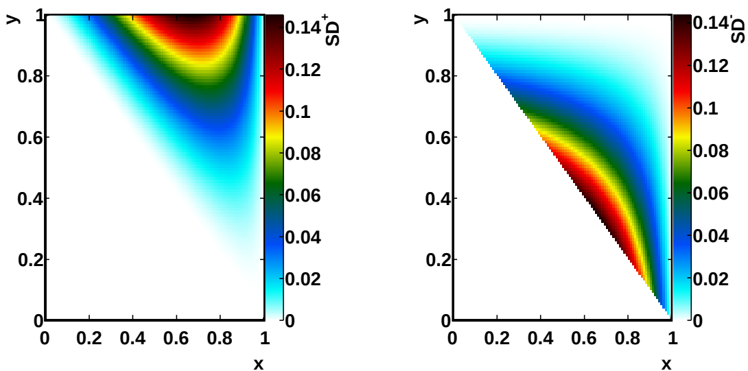
Figure 1: Components of the structure dependent terms of the decay width. Left: SD^+ , right: SD^-
