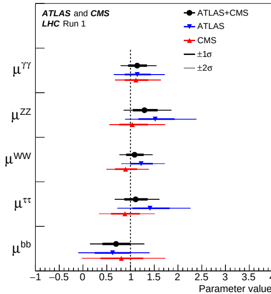
Figure 11.12: The signal strengths \mu measured by the ATLAS and CMS experiments [141] for the five principal Higgs boson decay channels assuming that the production cross sections are those of the SM.
