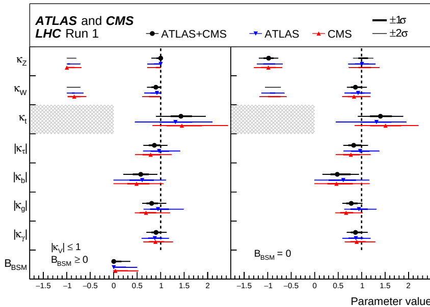
Figure 11.18: ATLAS-CMS combined measurements of coupling modifiers.
