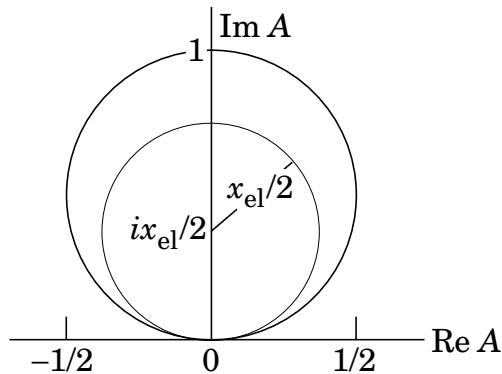
Figure 47.8: Argand plot for a resonance.
