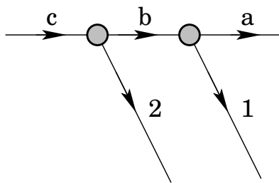
Figure 47.4: Particles participating in sequential two-body decay chain. Particles labeled 1 and 2 are visible while the particle terminating the chain (a) is invisible.
