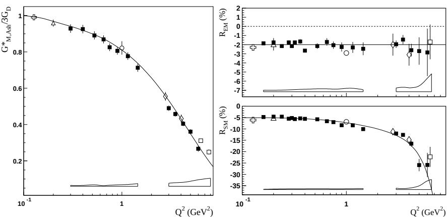
Figure 1: Left: The magnetic transition form factor for the \gamma^*p \rightarrow \Delta^+(1232) transition versus the photon virtuality Q^2 . Right: The electric and scalar quadrupole ratios R_{EM} and R_{SM} . The different symbols are results from different experiments at JLab (squares, diamonds, circle) and MAMI (triangle, cross). The boxes near the horizontal axis indicate model uncertainties of the squares. Curves to guide the eyes.
