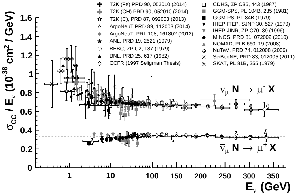
Figure 50.1: Measurements of \nu_\mu and \bar{\nu}_\mu CC inclusive scattering cross sections (per nucleon) divided by neutrino energy as a function of neutrino energy. Note the transition between logarithmic and linear scales occurring at 100 GeV. Neutrino cross sections are typically twice as large as their corresponding antineutrino counterparts, although this difference can be larger at lower energies. NC cross sections (not shown) are generally smaller but non-negligible compared to the CC scattering case.
