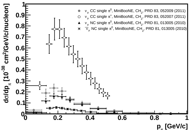
Figure 50.3: Differential cross sections for CC and NC pion production from MiniBooNE at a mean neutrino energy of 0.8 GeV. Shown here are the measurements as a function of the momentum of the outgoing pion in the interaction, a kinematic that is particularly sensitive to final state interactions. Other distributions are also available in the publications listed in the legend.
