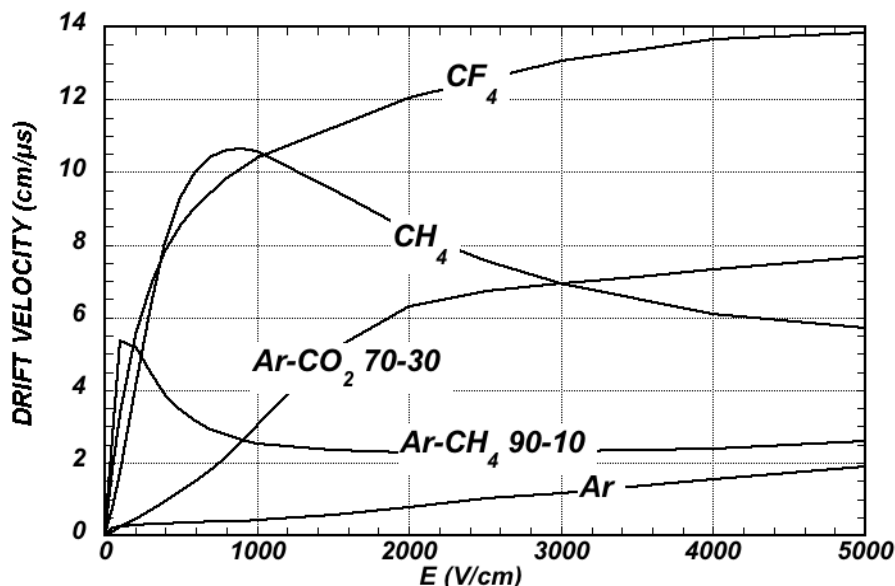
Figure 34.4: Computed electron drift velocity as a function of electric field in several gases at NTP and B = 0 [71].
