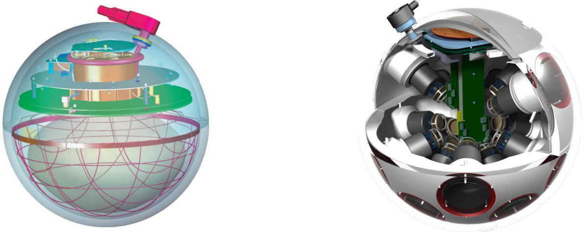
Figure 35.5: Schematic views of the digital OMs of IceCube (left) and KM3NeT (right).
