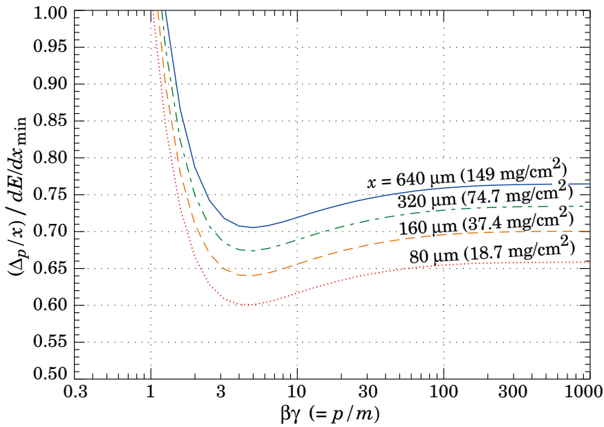
Figure 33.9: Most probable energy loss in silicon, scaled to the mean loss of a minimum ionizing particle, 388 eV/ \mu\text{m} (1.66 MeV g -1 cm 2 ).
