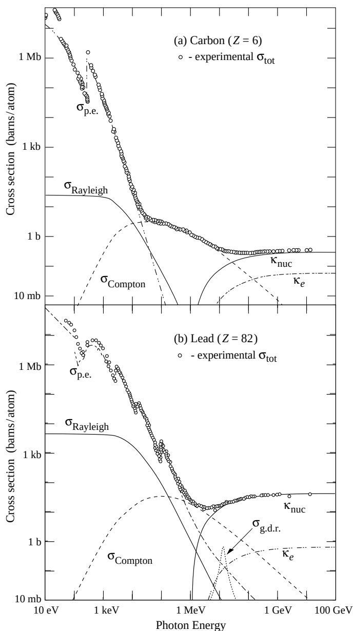
Figure 33.15: Photon total cross sections as a function of energy in carbon and lead, showing the contributions of different processes [51]:
