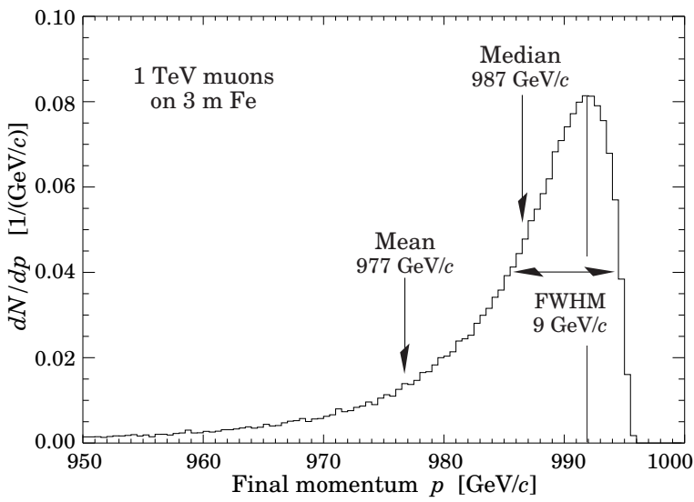
Figure 33.25: The momentum distribution of 1 TeV/c muons after traversing 3 m of iron as calculated with the MARS15 Monte Carlo code [72] by S.I. Striganov [5].
