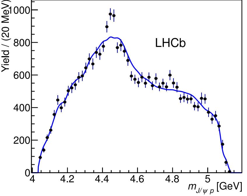
Figure 4: The efficiency-corrected and background-subtracted distribution of m_{J\psi p} for the data (black points with error bars), with the reflection of K^-p mass distribution and of the moments of the K^-p helicity angle, which can be accommodated by any plausible K^-p contribution (solid blue line) superimposed. The data and the reflection are inconsistent at > 9\sigma level.
