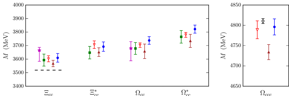
Figure 15.8: Comparison of lattice QCD results for the doubly and triply charmed baryon masses. Labels are Liu, et al. , [64]; Briceno, et al. , [65]; Namekawa, et al. , [66]; Padmanath, et al. , [67]; Alexandrou, et al. , [68]; and Brown, et al. , citequarkmod:Brown:2014ena. Only calculations with dynamical light quarks are included; for the doubly charmed baryons, only calculations were performed at or extrapolated to the physical pion mass are shown. Results without estimates of systematic uncertainties are labeled “stat. only”. The lattice spacing values used in the calculations are also given; a = 0 indicates that the results have been extrapolated to the continuum limit. In the plot of the doubly charmed baryons, the unconfirmed experimental result for the \Xi_{cc}^+ mass from SELEX [26,27] is shown with a dashed line.
