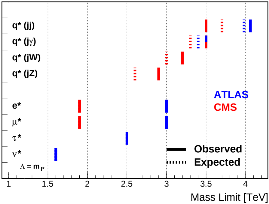
Figure 4: 95% C.L. lower mass limits for the excited quarks and leptons at ATLAS [65,67,69,70] and CMS [74,75,78,80] experiments. Shown are the most stringent limits for each excited fermion from both experiments. Only first generation quarks ( u , d ) with transition-magnetic type interactions with f_s = f = f' = 1 are considered for excited quarks, and the limits are shown for different final states denoted in parentheses. Excited lepton limits are given for contact interactions with \Lambda = m_{l^*} . The observed limit from q^* \rightarrow q + \gamma is 3.5 TeV for both ATLAS and CMS. For the excited leptons the observed and expected limits are same in both ATLAS and CMS.
