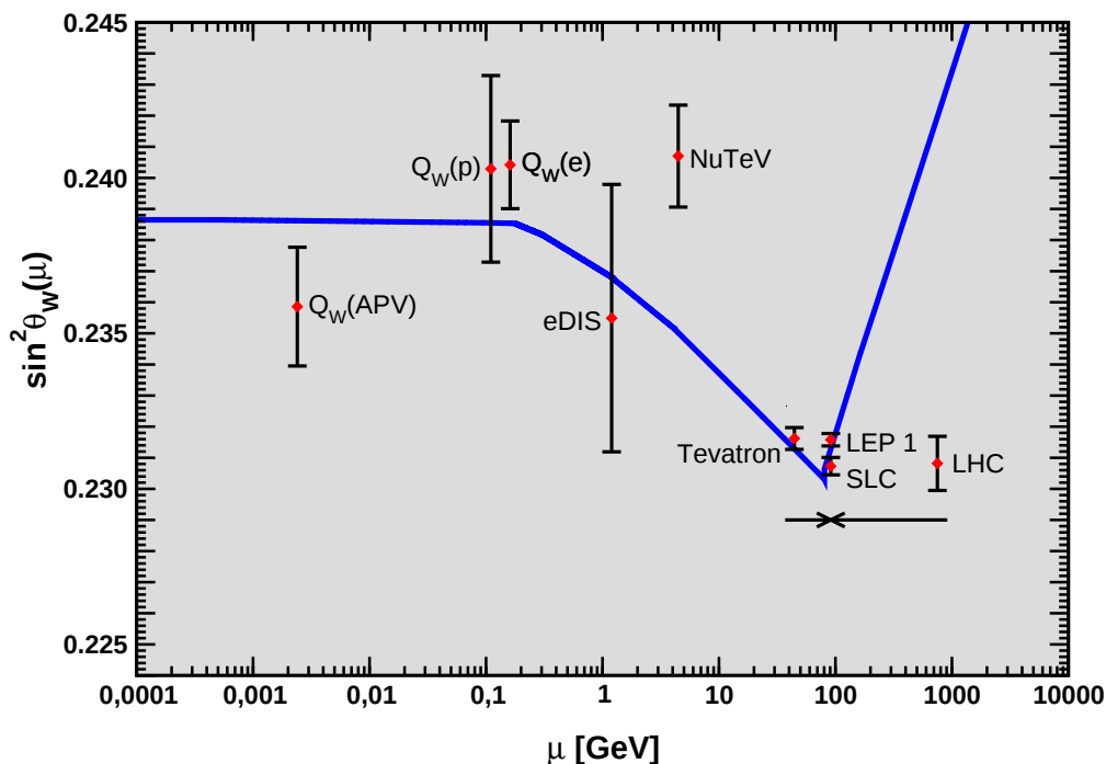
Figure 10.2: Scale dependence of the weak mixing angle defined in the \overline{\text{MS}} scheme [122] (for the scale dependence of the weak mixing angle defined in a mass-dependent renormalization scheme, see Ref. 123). The minimum of the curve corresponds to \mu = M_W , below which we switch to an effective theory with the W^\pm bosons integrated out, and where the \beta -function for the weak mixing angle changes sign. At the location of the W boson mass and each fermion mass there are also discontinuities arising from scheme dependent matching terms which are necessary to ensure that the various effective field theories within a given loop order describe the same physics. However, in the \overline{\text{MS}} scheme these are very small numerically and barely visible in the figure provided one decouples quarks at \mu = \hat{m}_q(\hat{m}_q) . The width of the curve reflects the theory uncertainty from strong interaction effects which at low energies is at the level of \pm 7 \times 10^{-5} [122]. Following the estimate [124] of the typical momentum transfer for parity violation experiments in Cs, the location of the APV data point is given by \mu = 2.4 MeV. For NuTeV we display the updated value from Ref. 125 and chose \mu = \sqrt{20} GeV which is about half-way between the averages of \sqrt{Q^2} for \nu and \bar{\nu} interactions at NuTeV. The Tevatron and LHC measurements are strongly dominated by invariant masses of the final state dilepton pair of \mathcal{O}(M_Z) and can thus be considered as additional Z pole data points. For clarity we displayed the Tevatron and LHC points horizontally to the left and to the right, respectively.
