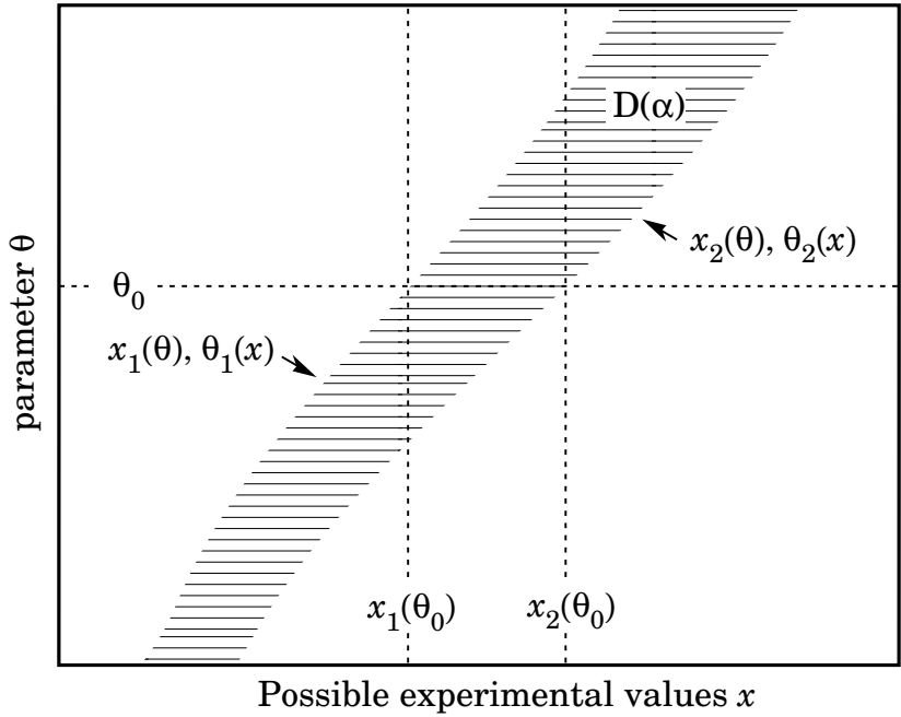
Figure 39.3: Construction of the confidence belt (see text).
