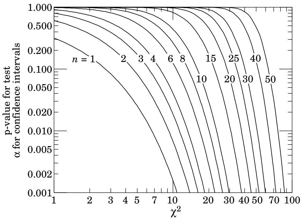
Figure 39.1: One minus the \chi^2 cumulative distribution, 1 - F(\chi^2; n) , for n degrees of freedom. This gives the p -value for the \chi^2 goodness-of-fit test as well as one minus the coverage probability for confidence regions (see Sec. 39.4.2.2).
