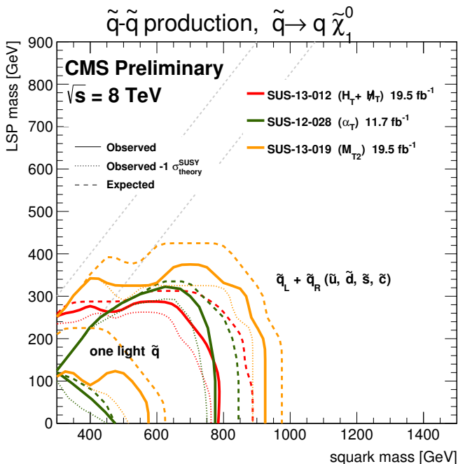
Figure 5: 95% C.L. exclusion contours in the squark-neutralino mass plane defined in the framework of simplified models assuming a single decay chain of \tilde{q} \rightarrow q \tilde{\chi}_1^0 [65]. Two assumptions for the squark pair production cross sections are displayed; a) eightfold degeneracy for the masses of the first and second generation squarks and b) only one light flavor squark.
