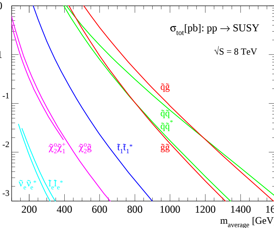
Figure 1: Cross sections for pair production of different particles as a function of their mass at the LHC for a center-of-mass energy of 8 TeV [52]. Typically the production cross section of colored squarks and gluinos is several orders of magnitude larger than the one for leptons or charginos. Except for the explicitly shown pair production of stops, production cross sections for squarks assumes mass degeneracy of left- and right-handed u , d , s , c and b squarks.
