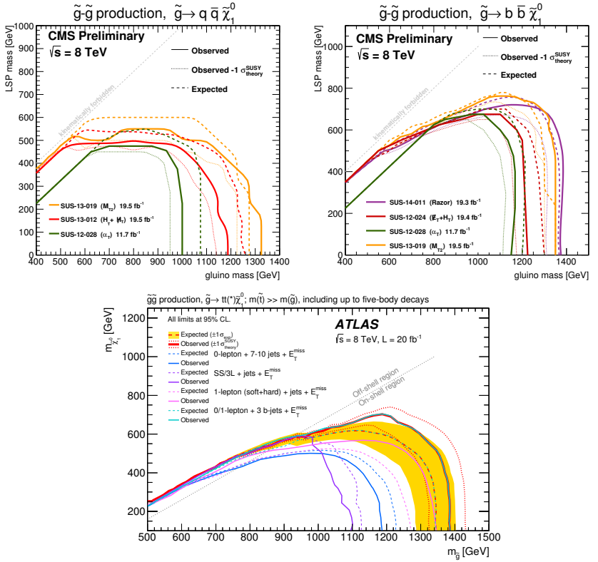
Figure 3: Upper mass limits, at 95% C.L., on gluino pair production for the decay chains \tilde{g} \rightarrow q \bar{q} \tilde{\chi}_1^0 (upper left) [65], \tilde{g} \rightarrow b \bar{b} \tilde{\chi}_1^0 (upper right) [66], and \tilde{g} \rightarrow t \bar{t} \tilde{\chi}_1^0 (lower middle) [62,157]. The limits are defined in the framework of simplified models assuming a single decay chain, (i.e. 100% branching fraction). The upper plots show limits from the CMS collaboration, while the displayed limits for \tilde{g} \rightarrow t \bar{t} \tilde{\chi}_1^0 are obtained from ATLAS searches. It should be note that the ATLAS results include both on-shell as well as off-shell production of gluino induced stop production (see text for details).
