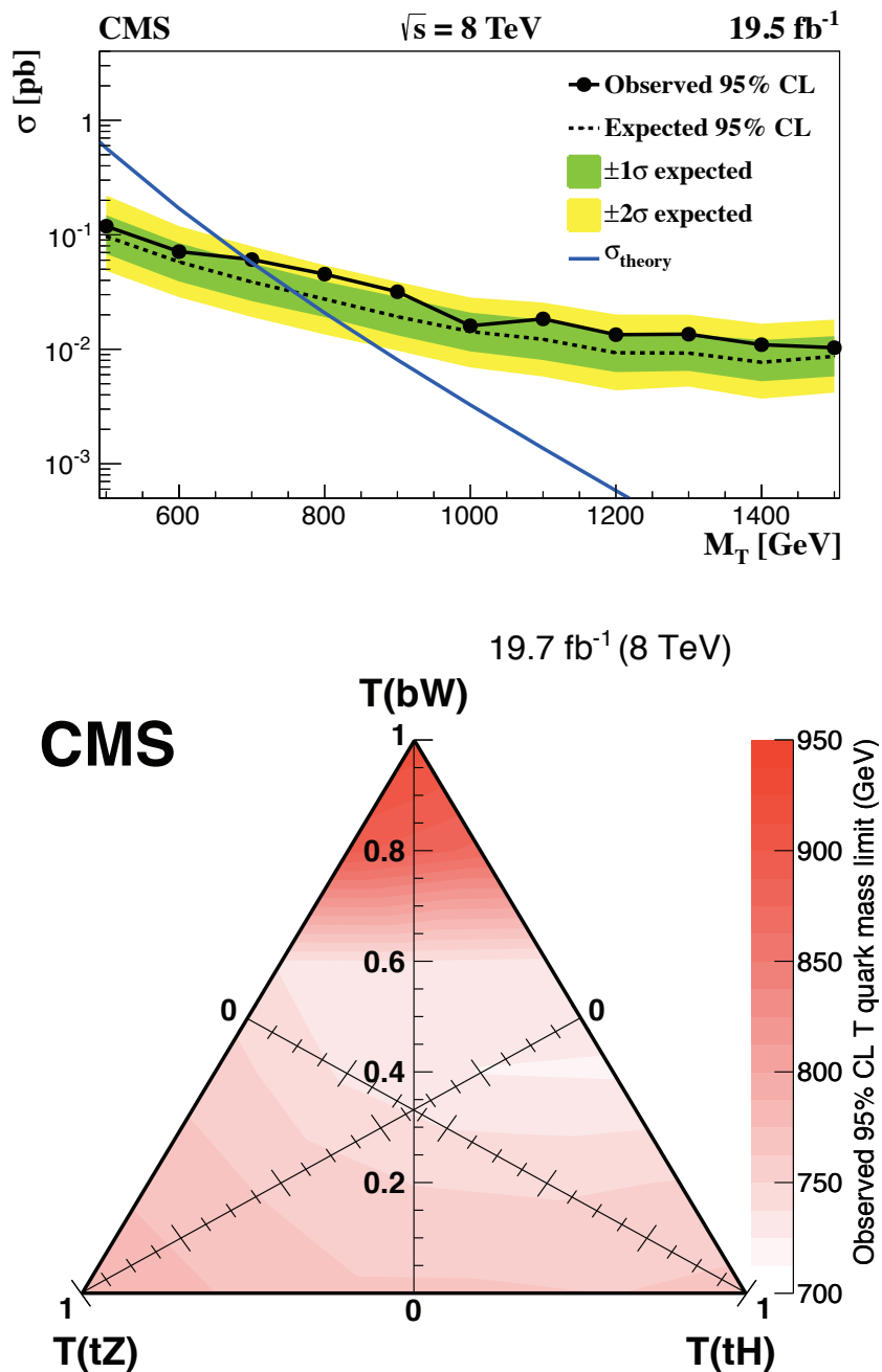
Figure 2: Top panel: upper limit on the T quark production cross section for branching fractions into bW , tH^0 , tZ of 50%, 25%, 25% obtained from the leptonic inclusive analysis [110]. Bottom panel: Branching fraction triangle with observed limits for the T quark mass from the CMS combination analysis [106].
