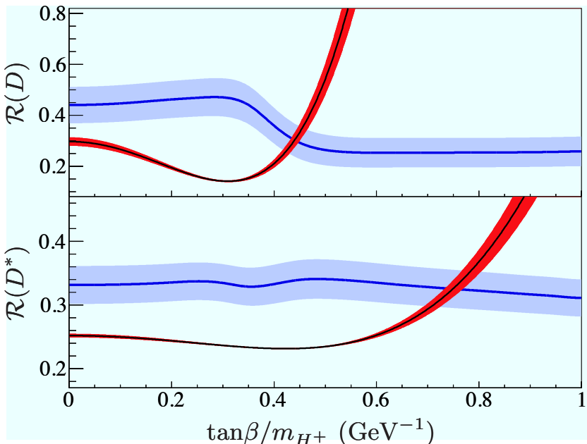
Figure 2: The \mathcal{R}_{D^{(*)}} measured in Ref. 151 along with expectations in the 2HDMII as a function of \tan\beta/m_{H+} .
