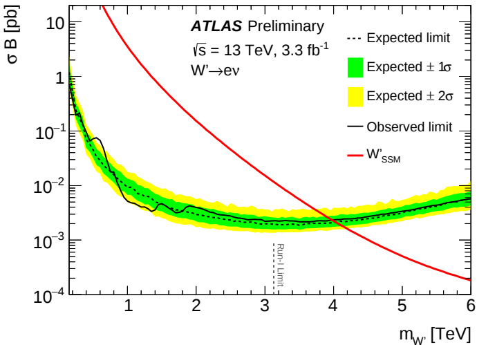
Figure 1: Upper limit on \sigma(pp \rightarrow W'X) B(W' \rightarrow e\nu) from ATLAS [20], at 95% CL. The red line shows the theoretical prediction in the Sequential SM.
