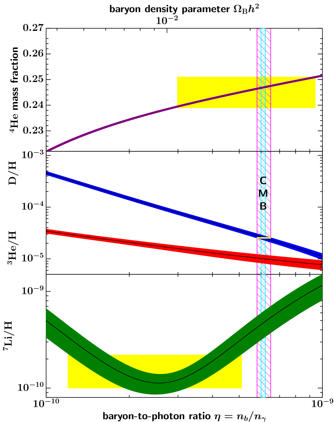
Figure 23.1: The primordial abundances of {}^4\text{He} , D, {}^3\text{He} , and {}^7\text{Li} as predicted by the standard model of Big-Bang nucleosynthesis — the bands show the 95% CL range [47]. Boxes indicate the observed light element abundances. The narrow vertical band indicates the CMB measure of the cosmic baryon density, while the wider band indicates the BBN D+ {}^4\text{He} concordance range (both at 95% CL).
