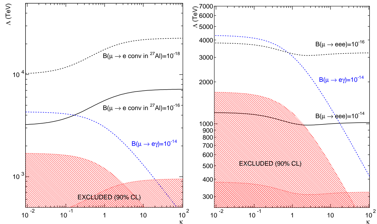
Figure 3: Model-independent CLFV sensitivities based on Eq (31a). Left panel shows the comparison of present constraints with prospective future sensitivities for \mu \rightarrow e\gamma and \mu \rightarrow e conversion. Right panel gives analogous comparison for \mu \rightarrow e\gamma and \mu \rightarrow 3e . Updated by [83] from Ref. [77].
