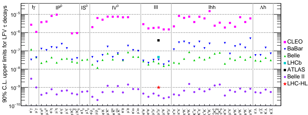
Figure 4: Current experimental limits on neutrinoless LFV \tau decays [86]. Also shown are the future projections at Belle-II [85] and at the HL-LHC [87].
