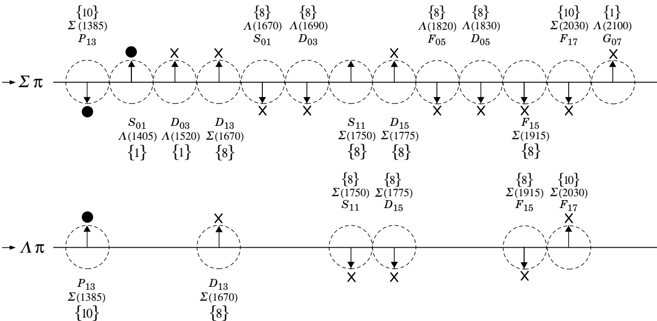
Figure 100.1: The signs of the imaginary parts of resonating amplitudes in the \bar{K}N \rightarrow \Lambda\pi and \Sigma\pi channels. The signs of the \Sigma(1385) and \Lambda(1405) , marked with a \bullet , are set by convention, and then the others are determined relative to them. The signs required by the SU(3) assignments of the resonances are shown with an arrow, and the experimentally determined signs are shown with an \times .
