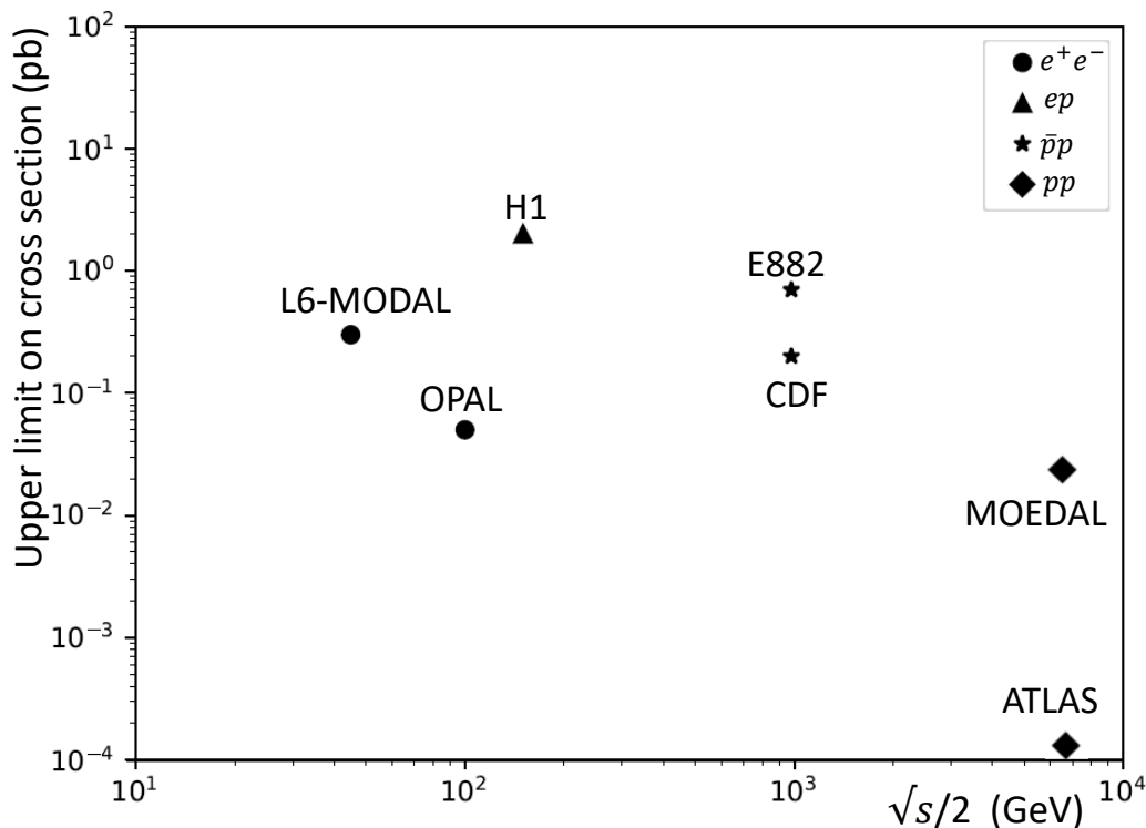
Figure 117.2: Upper limits on the production cross sections of monopoles from various collider-based experiments.
