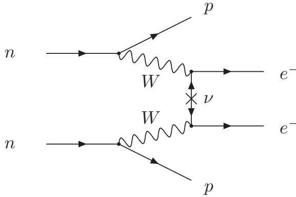
Figure 14.12: Feynman diagram for neutrinoless double-beta decay.
