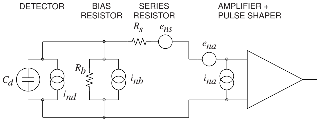
Figure 34.19: Equivalent circuit for noise analysis.
