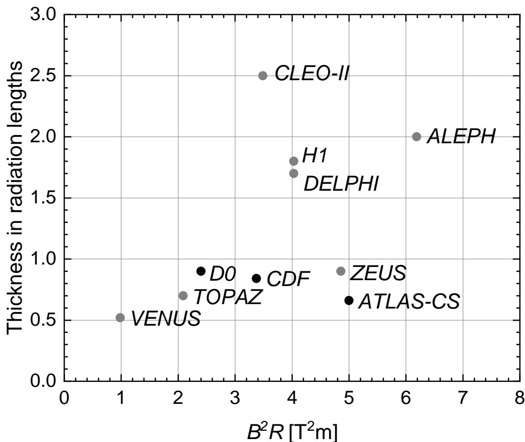
Figure 34.26: Magnet wall thickness in radiation length as a function of B^2R for various detector solenoids. Gray entries are for magnets no longer in use, and entries underlined are not listed in Table 34.11. Open circles are for magnets not designed to be “thin.” The SSC-SDC prototype provided important R&D for LHC magnets.
