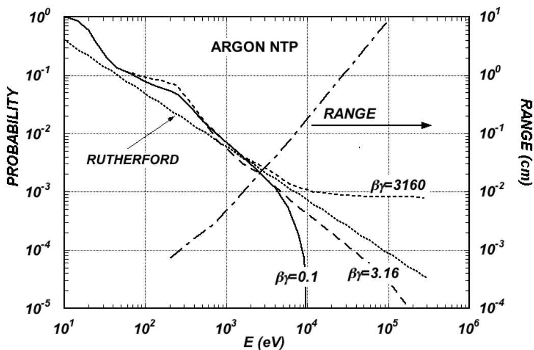
Figure 34.3: Probability of single collisions in which released electrons have an energy E or larger (left scale) and practical range of electrons in Ar/CH 4 (P10) at NTP (dot-dashed curve, right scale) [88].
