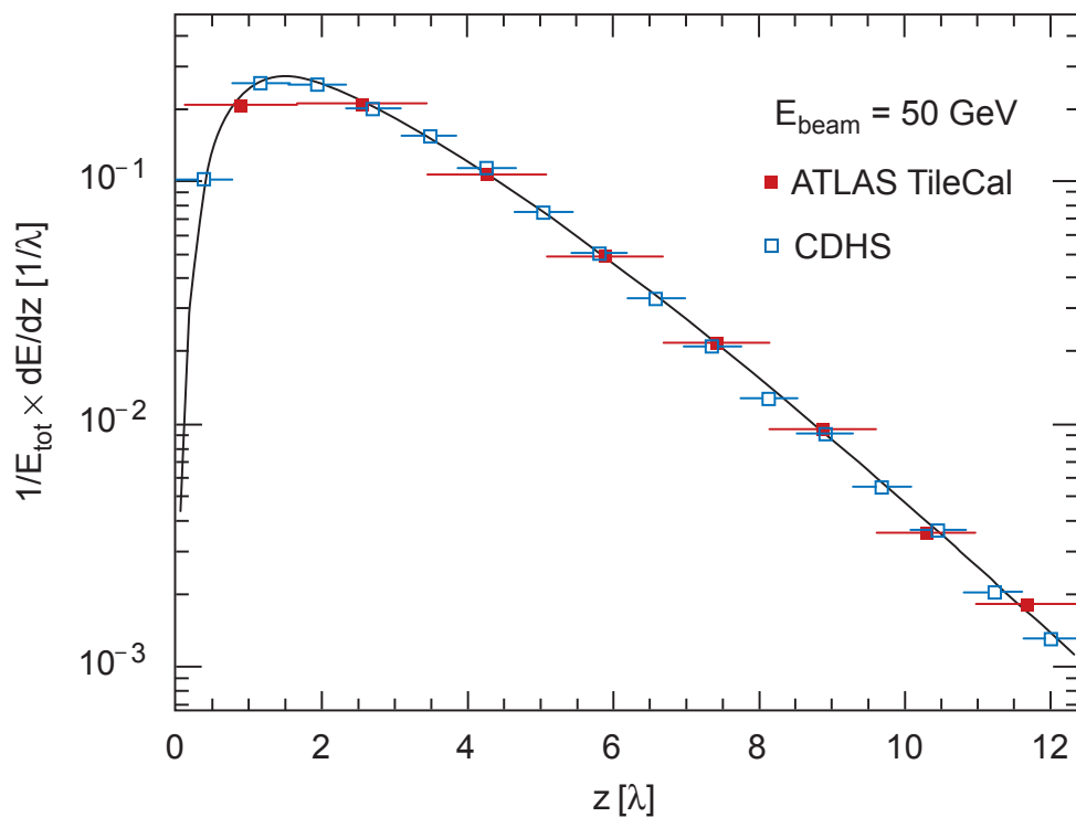
Figure 34.24: Mean profiles of \pi^+ (mostly) induced cascades in the CDHS neutrino detector [256] and in the ATLAS tile calorimeter [225]. Measurements are front of the calorimeter, and so are convoluted with the first interaction distance.
