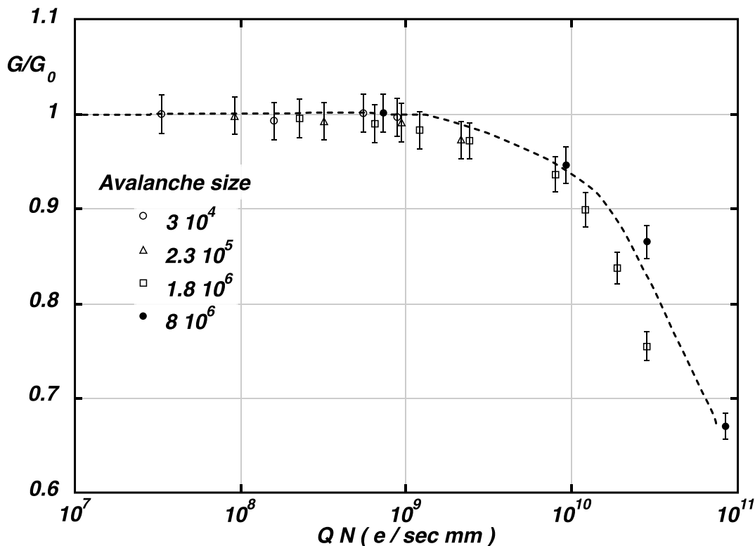
Figure 34.8: Charge rate dependence of normalized gas gain G/G_0 (relative to zero counting rate) in proportional thin-wire detectors [111]. Q is the total charge in single avalanche; N is the particle rate per wire length.
