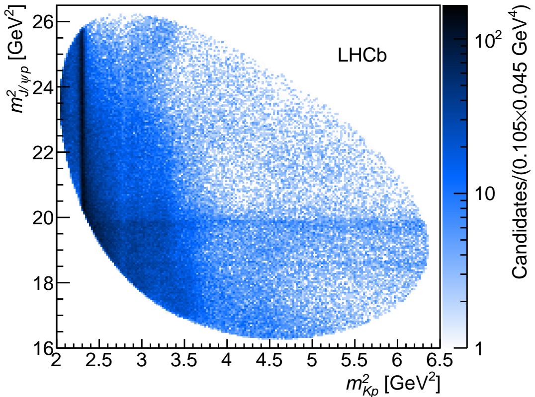
Figure 106.1: Dalitz plot distributions for \Lambda_b^0 \rightarrow J/\psi p K^- decays as observed by LHCb.
