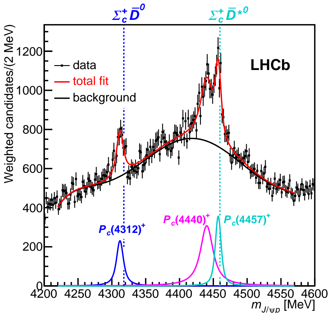
Figure 106.2: Fit to the J/\psi p mass distribution, in which events were weighted to suppress \Lambda^* \rightarrow pK^- backgrounds, of three Breit-Wigner functions and a sixth-order polynomial background. This fit was used to determine the central values of the masses and widths of the P_c^+ states reported by LHCb. The mass thresholds for the \Sigma_c^+ \bar{D}^0 and \Sigma_c^+ \bar{D}^{*0} final states are superimposed.
