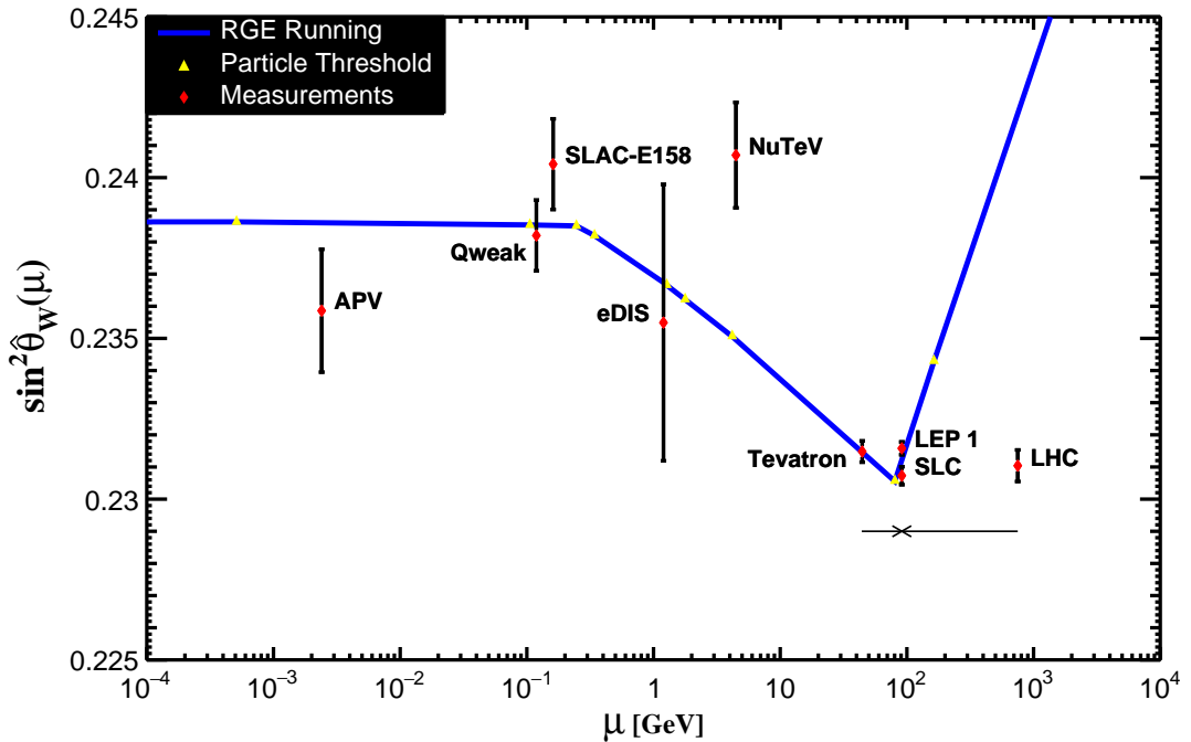
Figure 10.2: Scale dependence of the weak mixing angle defined in the \overline{\text{MS}} scheme [102,103] (for the scale dependence of the weak mixing angle defined in a mass-dependent renormalization scheme, see [101]). The minimum of the curve corresponds to \mu = M_W , below which we switch to an effective theory with the W^\pm bosons integrated out, and where the \beta -function for the weak mixing angle changes sign. At the location of the W boson mass and each fermion mass there are also discontinuities arising from scheme dependent matching terms which are necessary to ensure that the various effective field theories within a given loop order describe the same physics. However, in the \overline{\text{MS}} scheme these are very small numerically and barely visible in the figure provided one decouples quarks at \mu = \hat{m}_q(\hat{m}_q) . The width of the curve exceeds the theory uncertainty from strong interaction effects which at low energies is at the level of \pm 2 \times 10^{-5} [103]. Following the estimate [104] of the typical momentum transfer for parity violation experiments in Cs, the location of the APV data point is given by \mu = 2.4 MeV. For NuTeV we display the updated value from [105] and chose \mu = \sqrt{20} GeV which is about half-way between the averages of \sqrt{Q^2} for \nu and \bar{\nu} interactions at NuTeV. The Tevatron and LHC measurements are strongly dominated by invariant masses of the final state dilepton pair of \mathcal{O}(M_Z) and can thus be considered as additional Z pole data points. For clarity we displayed the Tevatron and LHC points horizontally to the left and to the right, respectively.
