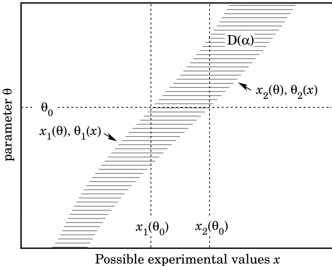
Figure 39.3: Construction of the confidence belt (see text).
