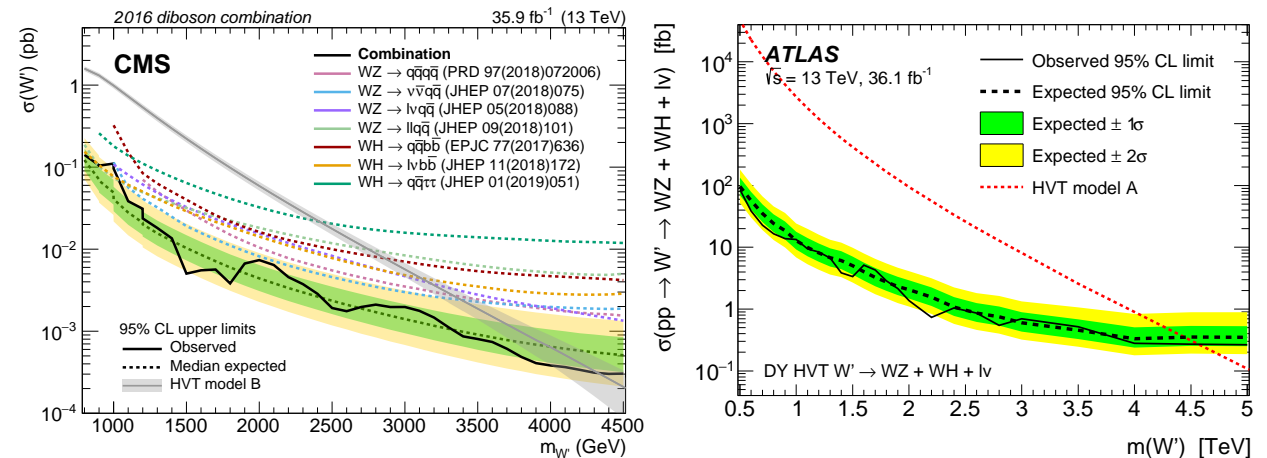
Figure 114.2: Left panel: Observed limits from W' to diboson from CMS [89]. Right panel: Observed limits from W' to diboson decays from ATLAS [88].
