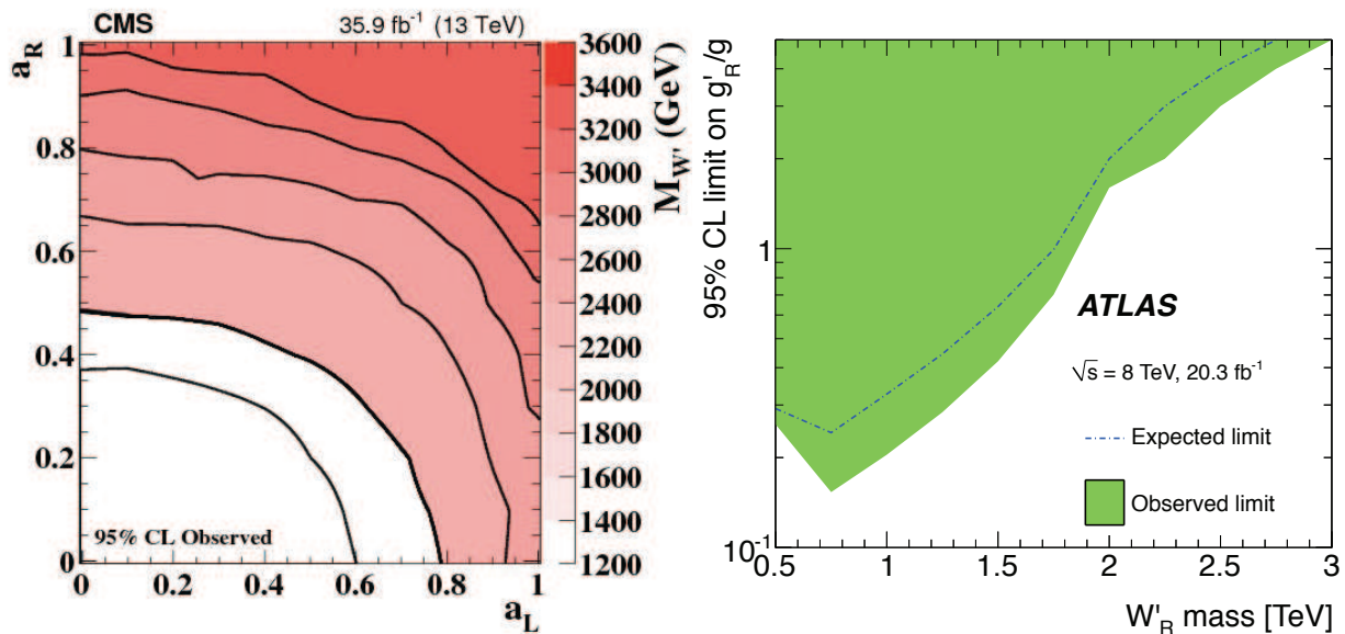
Figure 114.1: Left panel: Observed limits on the W' boson mass as function of the left-handed ( a_L ) and right-handed ( a_R ) couplings. Black lines represent contours of equal W' boson mass [82]. Right panel: Observed and expected regions, on the g'/g vs mass of the W' boson plane, that are excluded at 95% CL, for right-handed W' bosons [86].
