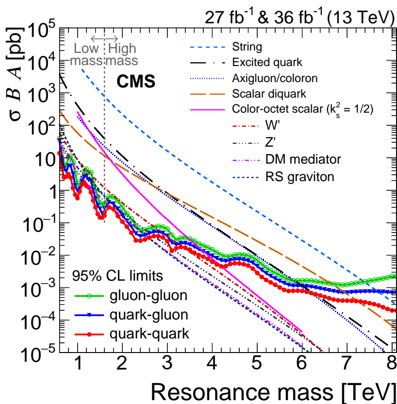
Figure 114.5: Observed 95% C.L. limits on \sigma \times B \times A for string resonances, excited quarks, axigluons, colorons, E6 diquarks, s8 resonances, W' and Z' bosons, and Randall-Sundrum Gravitons g_{KK} from [145].
