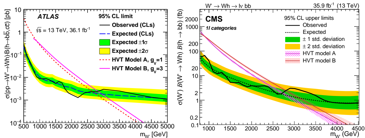
Figure 108.2: Upper limits on W' production cross section times branching fraction into a W and a SM Higgs boson decaying into heavy-flavor quarks, from ATLAS [37] (left) and CMS [38] (right).
