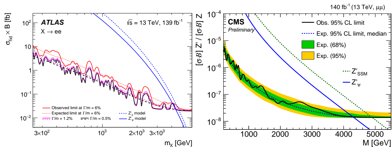
Figure 109.1: Upper limits on the cross section for Z' production times the branching fraction for Z' \rightarrow e^+e^- (left panel, set by ATLAS [20]) or Z' \rightarrow \mu^+\mu^- (right panel, set by CMS [21]) as a function of M_{Z'} . The lines labelled by Z'_\psi and Z'_\chi are theoretical predictions for the U(1)_{10+x5} models in Table 109.1 with x = -3 and x = +1 , respectively, for g_z fixed by an E_6 unification condition. The Z'_{\text{SSM}} line corresponds to Z' couplings equal to those of the Z boson.
