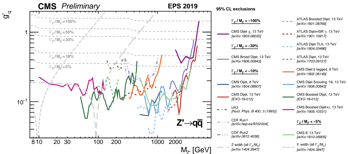
Figure 109.2: Upper limits on the Z' coupling to quarks as a function of M_{Z'} based on various searches performed by the ATLAS, CMS, CDF, and UA2 experiments [28].
