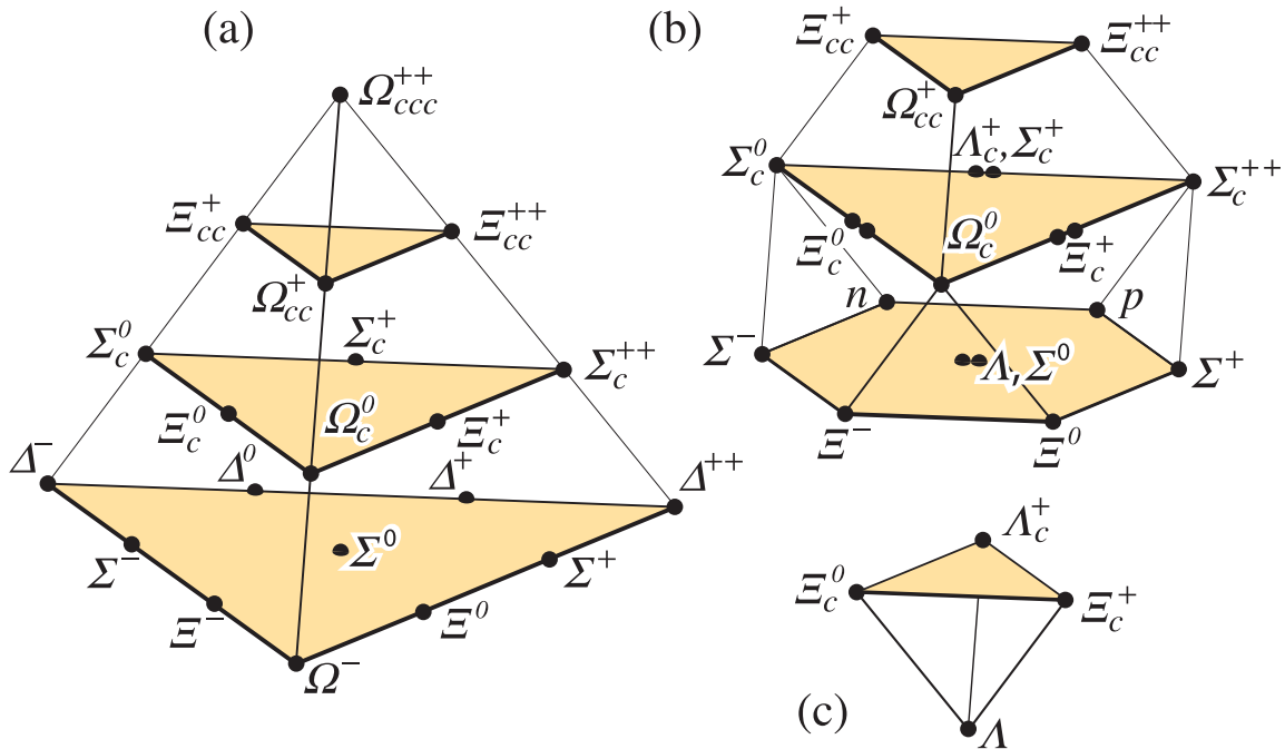
Figure 105.2: SU(4) multiplets of baryons made of u , d , s , and c quarks. (a) The 20-plet with an SU(3) decuplet on the lowest level. (b) The 20'_1 -plet with an SU(3) octet on the lowest level. (c) The \bar{4} -plet. Note that here and in Fig. 105.3, but not in Fig. 105.1, each charge state is shown separately.
