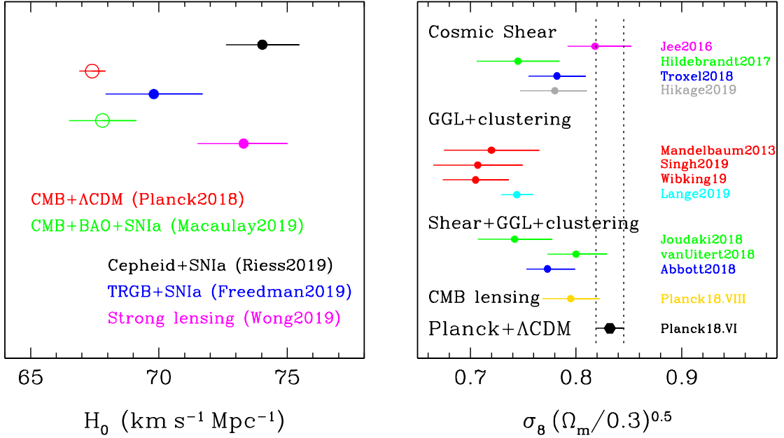
Figure 27.3: Tensions between low-redshift cosmological measurements and the predictions of a CMB-normalized \Lambda CDM model. All error bars are 1\sigma ; see text for observational references. ( Left ) Open circles show values of H_0 for flat \Lambda CDM with Planck parameters or a general dark energy model constrained by a combination of CMB, BAO, and supernova data. Filled circles show distance-ladder estimates based on Cepheid or TRGB calibration or an independent estimate using gravitational-lens time delays. ( Right ) Matter clustering characterized by the parameter combination \sigma_8(\Omega_m/0.3)^{0.5} , as predicted by a Planck -normalized \Lambda CDM model (vertical dotted lines, black hexagon) and estimated from weak gravitational lensing using cosmic shear, galaxy-galaxy lensing and galaxy clustering, or a combination of the two constraints. Points of the same color are based on the same weak-lensing data. The “CMB lensing” point shows the value of \sigma_8 for \Omega_m = 0.3 inferred from Planck CMB lensing, a measurement that is independent of the “Planck+ \Lambda CDM” prediction and weighted to somewhat higher redshift than the other weak-lensing points.
