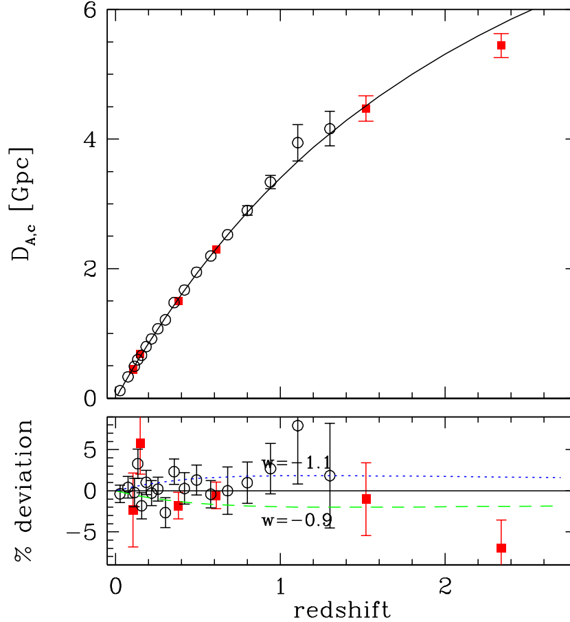
Figure 27.1: Distance-redshift relation measured from Type Ia SNe and BAO compared to the predictions (black curve) of a flat \Lambda CDM model with \Omega_m = 0.315 and h = 0.674 , the best-fit parameters inferred from Planck CMB data [33]. Circles show binned luminosity distances from the JLA SN sample [35], multiplied by (1+z)^{-1} to convert to comoving angular diameter distance. Red squares show BAO distance measurements from the 6dFGS, SDSS-II, BOSS, and eBOSS surveys (see text for details and references). The lower panel plots residuals from the \Lambda CDM prediction, with dashed and dotted curves that show the effect of changing w by \pm 0.1 while all other parameters are held fixed. Note that the SN data points can be shifted up or down by a constant factor to account for freedom in the peak luminosity, while the BAO points are calibrated to 0.2% precision by the sound horizon scale computed from Planck data. The errors on the BAO data points are approximately independent. In the upper panel, error bars are plotted only at z > 0.7 to avoid visual confusion.
