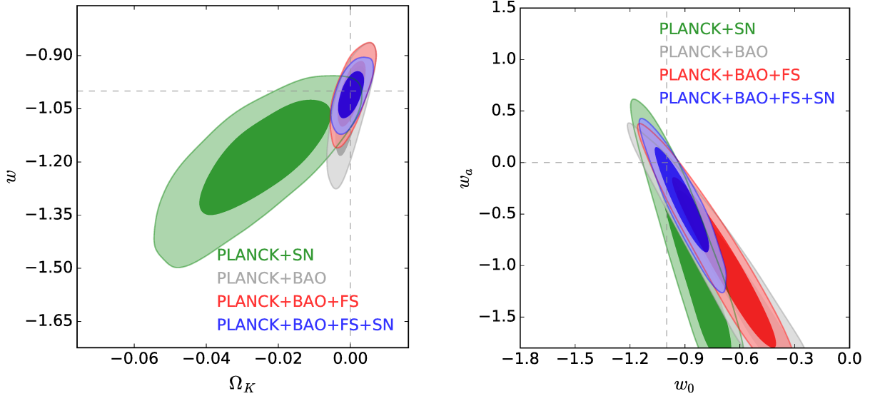
Figure 27.2: Constraints on dark energy model parameters from combinations of CMB, BAO, galaxy clustering, and supernova (SN) data, taken from Ref. [42]. The left panel shows 68% and 95% confidence contours in the \text{owCDM} model, with constant equation-of-state parameter w and non-zero space curvature \Omega_K \equiv 1 - \Omega_{\text{tot}} . Green and gray contours show the combination of Planck CMB data with SN or BAO data, respectively. Red contours combine CMB, BAO, and the full shape (FS) of redshift-space galaxy clustering. Blue contours add SN data to this combination. The right panel shows confidence contours for the same data combinations in the w_0w_a\text{CDM} model, which assumes a flat Universe and an evolving equation of state with w(a) = w_0 + w_a(1 - a) .
