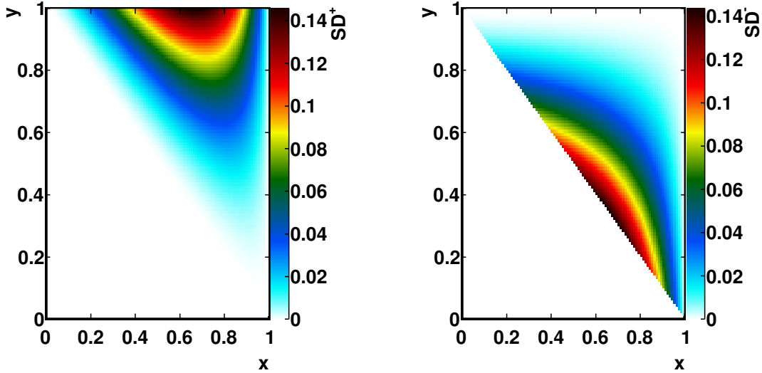
Figure 68.1: Components of the structure dependent terms of the decay width. Left: \text{SD}^+ , right: \text{SD}^-
