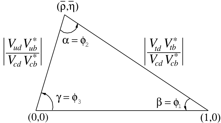
Figure 12.1: Sketch of the unitarity triangle.
