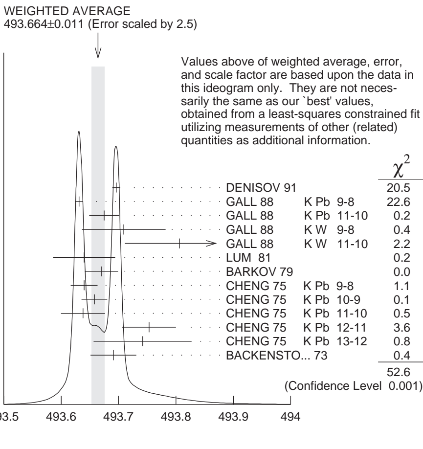
Figure 1: Ideogram of m_{K^\pm} mass measurements. GALL 88 and CHENG 75 measurements are shown separately for each transition they measured.
