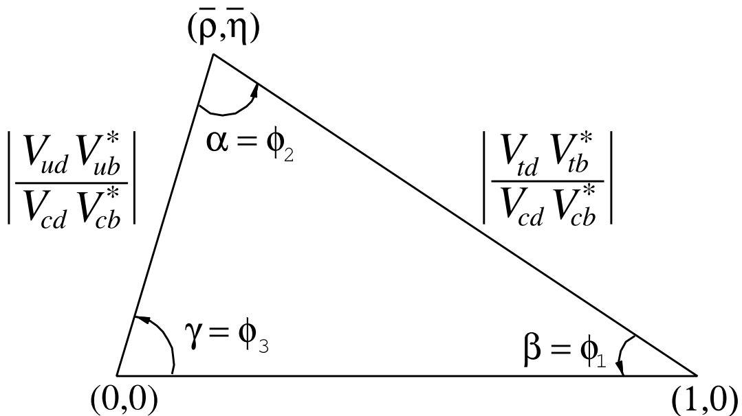
Figure 12.1: Sketch of the unitarity triangle.
