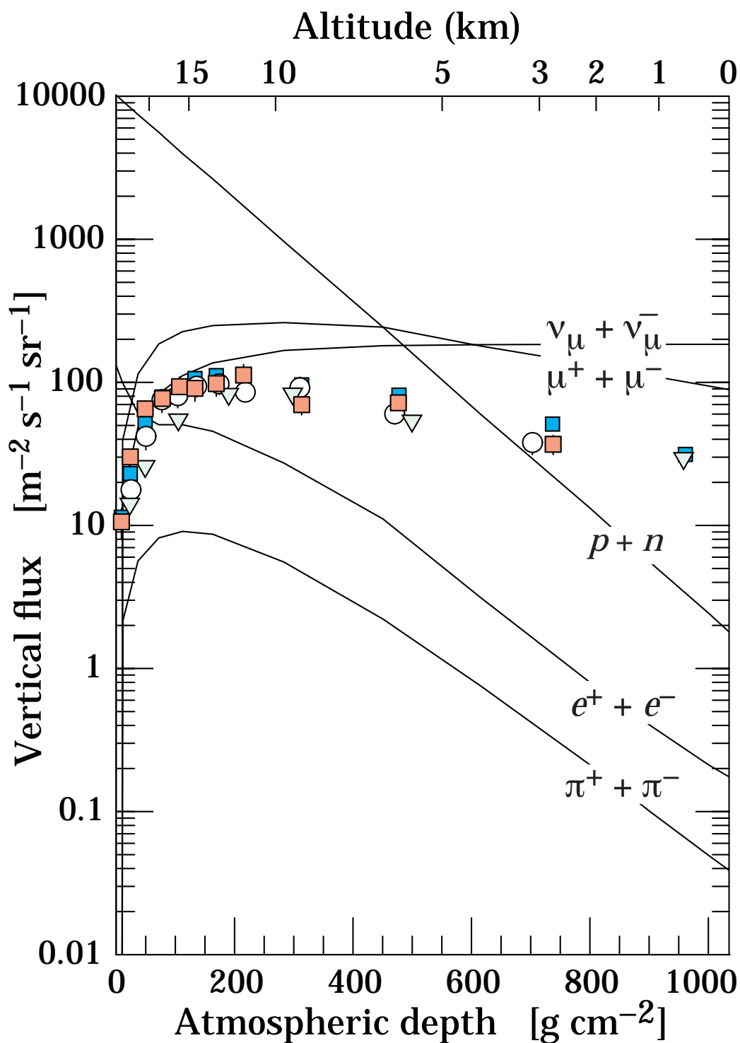
Figure 30.4: Vertical fluxes of cosmic rays in the atmosphere with E > 1 \text{ GeV} estimated from the nucleon flux of Eq. (30.2). The points show measurements of negative muons with E_{\mu} > 1 \text{ GeV} [46–51].
