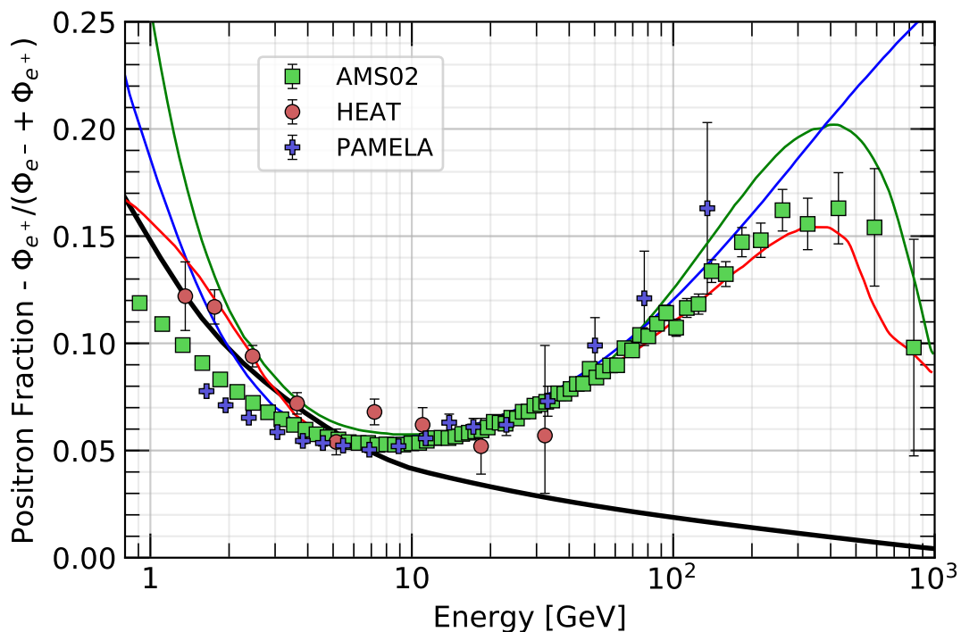
Figure 30.3: The positron fraction (ratio of the flux of e^+ to the total flux of e^+ and e^- ) [22,30–32]. The heavy black line is a model of pure secondary production [33] and the three thin lines show three representative attempts to model the positron excess with different phenomena: green: dark matter decay [34]; blue: propagation physics [35]; red: production in pulsars [36]. The ratio below 10 GeV is dependent on the polarity of the solar magnetic field.
