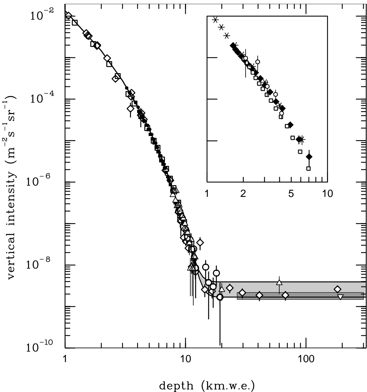
Figure 30.7: Vertical muon intensity vs depth (1 km.w.e. = 10^5 g cm ^{-2} of standard rock). The experimental data are from: \diamond : the compilations of Crouch [73], \square : Baksanu [74], \circ : LVD [75], \bullet : MACRO [76], \blacksquare : Frejus [77], and \triangle : SNO [78]. The shaded area at large depths represents neutrino-induced muons of energy above 2 GeV. The upper line is for horizontal neutrino-induced muons, the lower one for vertically upward muons. Darker shading shows the muon flux measured by the SuperKamiokande experiment. The inset shows the vertical intensity curve for water and ice published in Refs. [79–82]. Additional data extending to slant depths of 13 km are available in [83].
