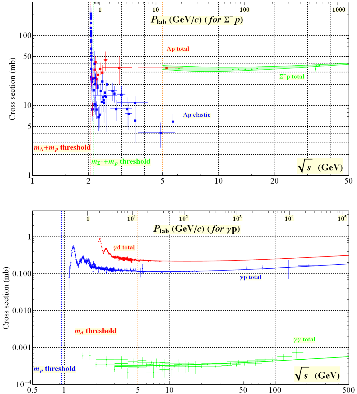
Figure 52.11: Total and elastic cross sections for \Lambda p , total cross section for \Sigma^- p , and total hadronic cross sections for \gamma d , \gamma p , and \gamma\gamma collisions as a function of laboratory beam momentum and the total center-of-mass energy. Corresponding computer-readable data files may be found at http://pdg.lbl.gov/current/xsect/ . (Courtesy of the COMPAS group, NRC KI – IHEP, Protvino, August 2019.)
