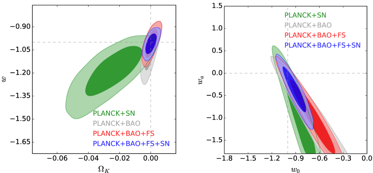
Figure 28.2: Constraints on dark energy model parameters from combinations of CMB, BAO, galaxy clustering, and supernova (SN) data, taken from Ref. [38]. The left panel shows 68% and 95% confidence contours in the \omega wCDM model, with constant equation-of-state parameter w and non-zero space curvature \Omega_K \equiv 1 - \Omega_{\text{tot}} . Green and gray contours show the combination of Planck CMB data with SN or BAO data, respectively. Red contours combine CMB, BAO, and the full shape (FS) of redshift-space galaxy clustering. Blue contours add SN data to this combination. The right panel shows confidence contours for the same data combinations in the w_0 w_a CDM model, which assumes a flat Universe and an evolving equation of state with w(a) = w_0 + w_a(1 - a) .
