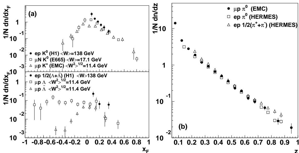
Figure 19.9: (a) 1/N \cdot dn/dx_F for identified strange particles in DIS at various values of W [171, 174, 179]. (b) 1/N \cdot dn/dz for measurements of pions in fixed-target DIS experiments [172, 175, 178].
